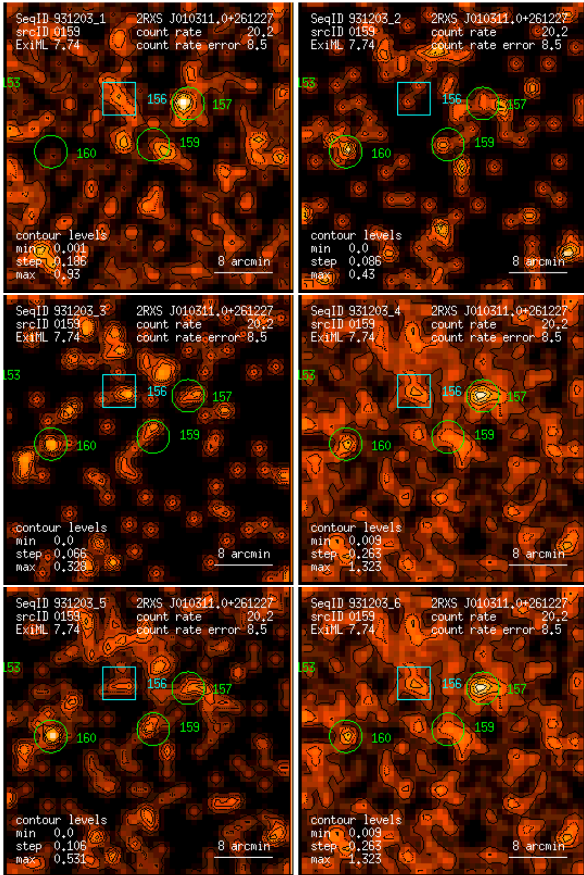
Figure 159: RASS 931203: detection 0159: band rate images, Gaussian filter: (1) PSPC channels 11 – 41, (2) 52 – 90, (3) 91 – 201, (4) 11 – 235, (5) 52 – 201, (6) 11 – 201. Broad band rates in counts/ks. Band rate contour levels in counts/ks/arcmin 2 .
