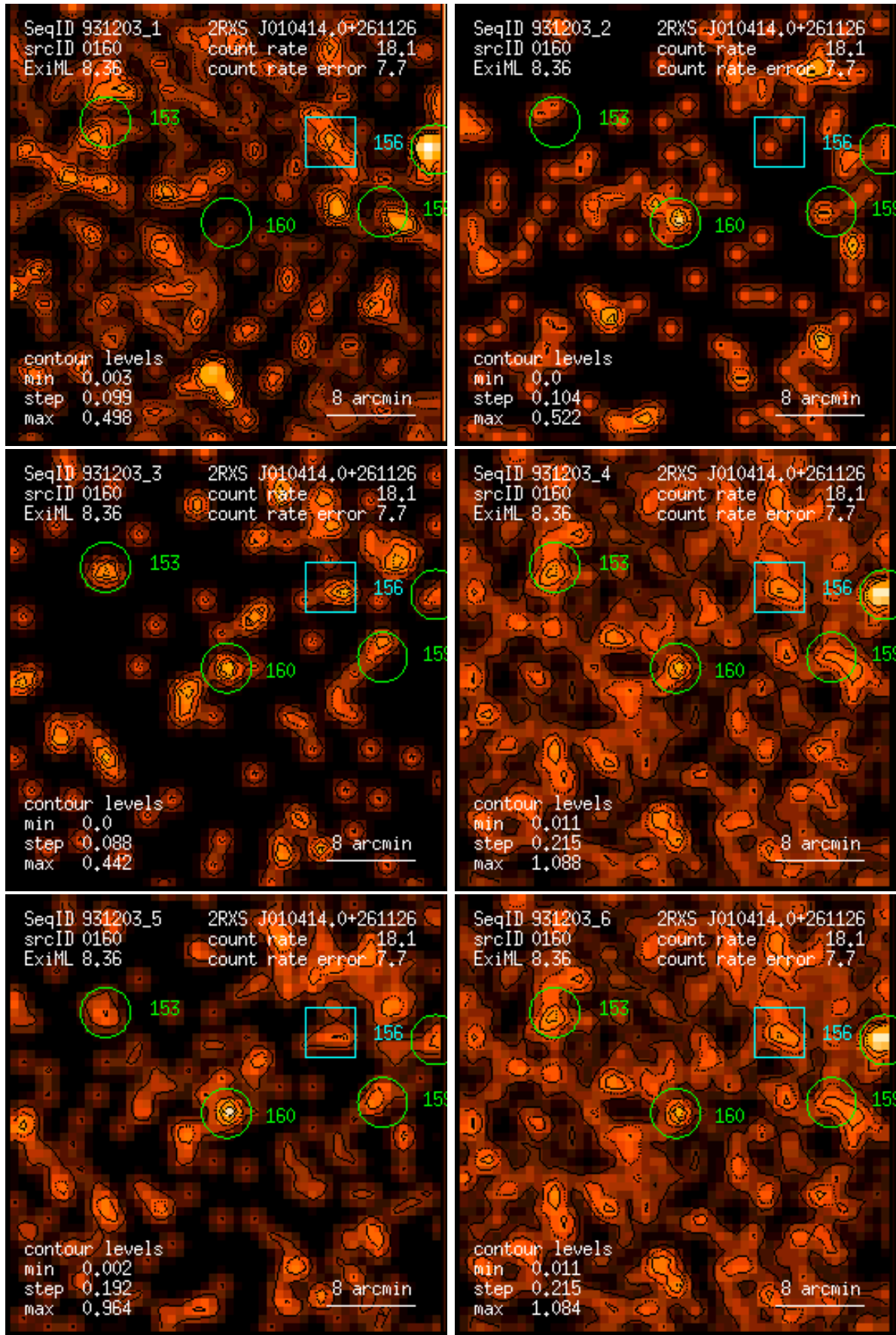
Figure 160: RASS 931203: detection 0160: band rate images, Gaussian filter: (1) PSPC channels 11 – 41, (2) 52 – 90, (3) 91 – 201, (4) 11 – 235, (5) 52 – 201, (6) 11 – 201. Broad band rates in counts/ks. Band rate contour levels in counts/ks/arcmin 2 .
