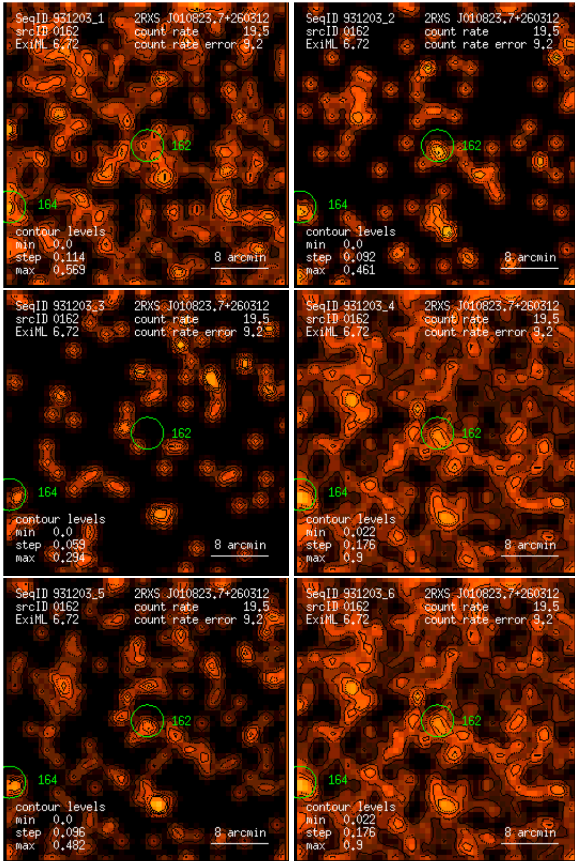
Figure 162: RASS 931203: detection 0162: band rate images, Gaussian filter: (1) PSPC channels 11 – 41, (2) 52 – 90, (3) 91 – 201, (4) 11 – 235, (5) 52 – 201, (6) 11 – 201. Broad band rates in counts/ks. Band rate contour levels in counts/ks/arcmin 2 .
