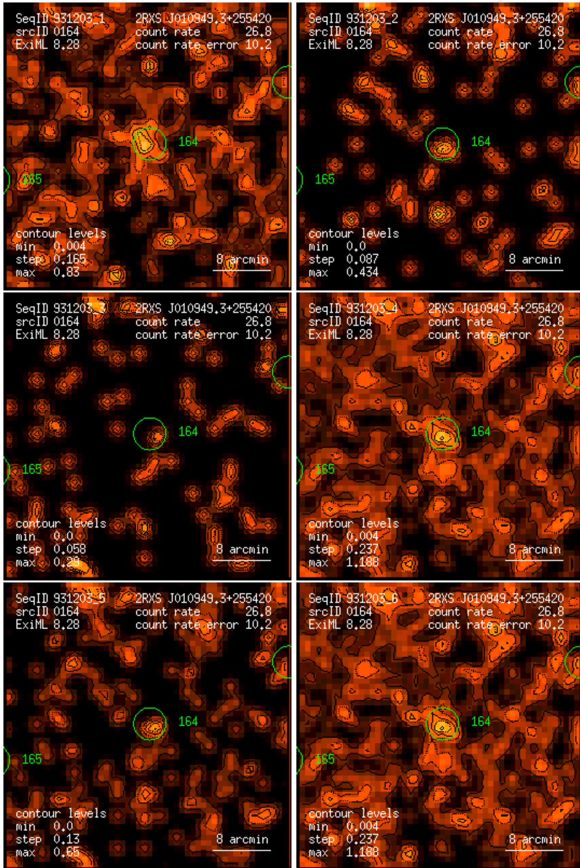
Figure 164: RASS 931203: detection 0164: band rate images, Gaussian filter: (1) PSPC channels 11 – 41, (2) 52 – 90, (3) 91 – 201, (4) 11 – 235, (5) 52 – 201, (6) 11 – 201. Broad band rates in counts/ks. Band rate contour levels in counts/ks/arcmin 2 .
