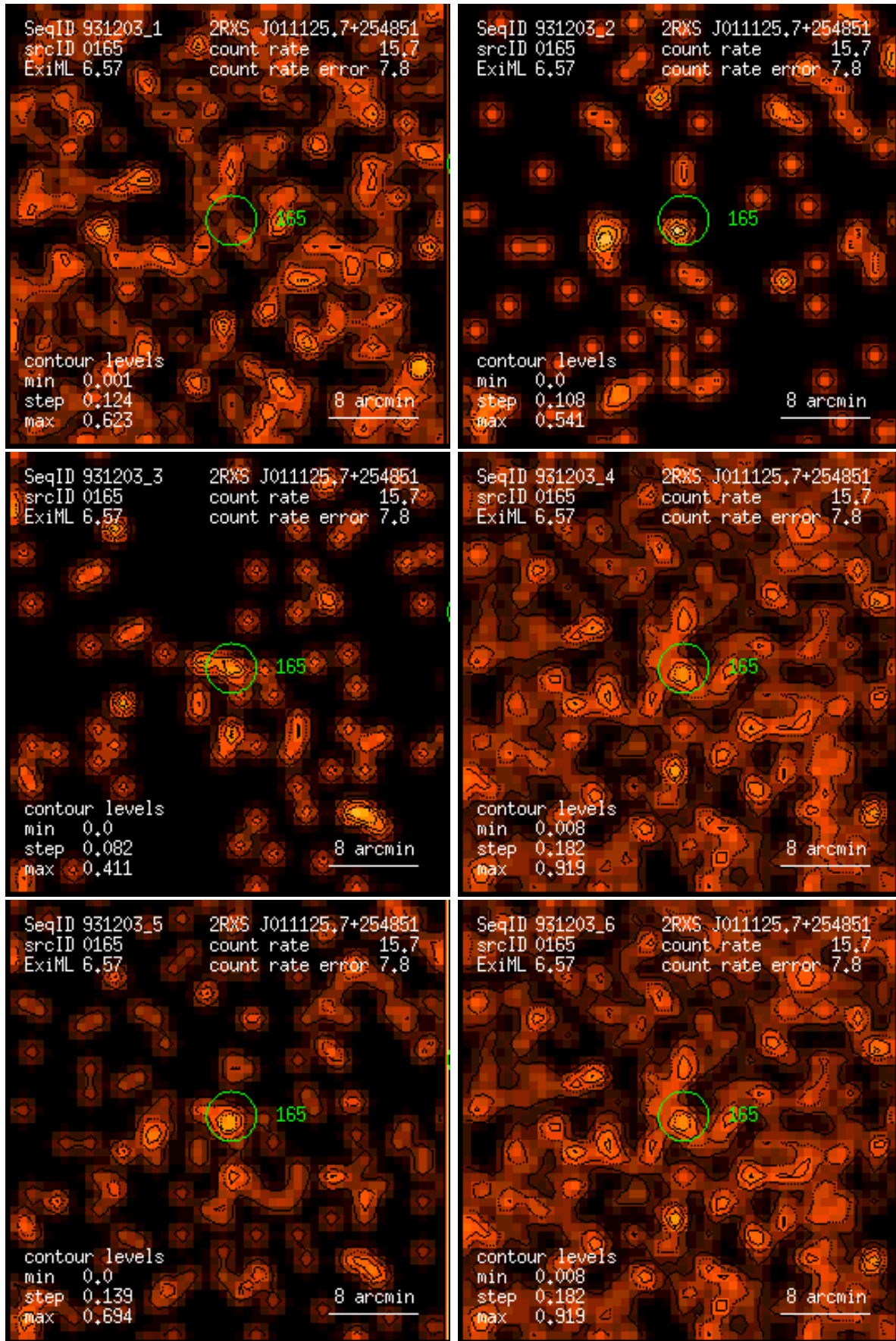
Figure 165: RASS 931203: detection 0165: band rate images, Gaussian filter: (1) PSPC channels 11 – 41, (2) 52 – 90, (3) 91 – 201, (4) 11 – 235, (5) 52 – 201, (6) 11 – 201. Broad band rates in counts/ks. Band rate contour levels in counts/ks/arcmin 2 .
