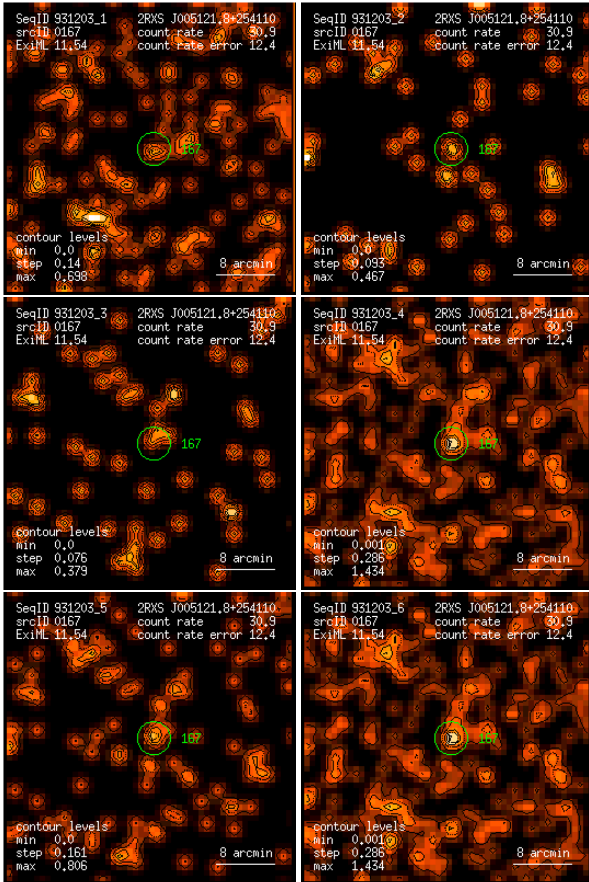
Figure 167: RASS 931203: detection 0167: band rate images, Gaussian filter: (1) PSPC channels 11 – 41, (2) 52 – 90, (3) 91 – 201, (4) 11 – 235, (5) 52 – 201, (6) 11 – 201. Broad band rates in counts/ks. Band rate contour levels in counts/ks/arcmin 2 .
