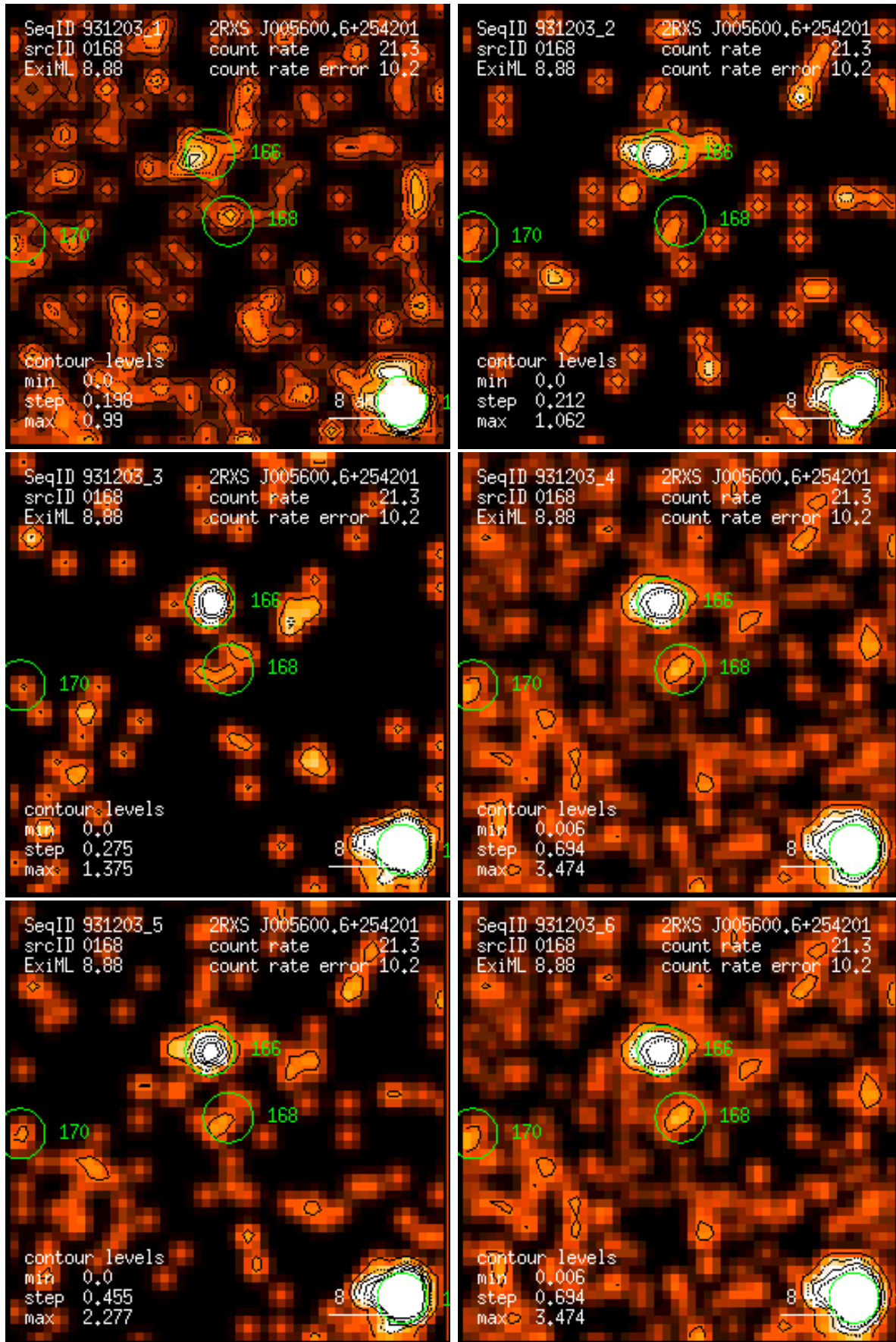
Figure 168: RASS 931203: detection 0168: band rate images, Gaussian filter: (1) PSPC channels 11 – 41, (2) 52 – 90, (3) 91 – 201, (4) 11 – 235, (5) 52 – 201, (6) 11 – 201. Broad band rates in counts/ks. Band rate contour levels in counts/ks/arcmin 2 .
