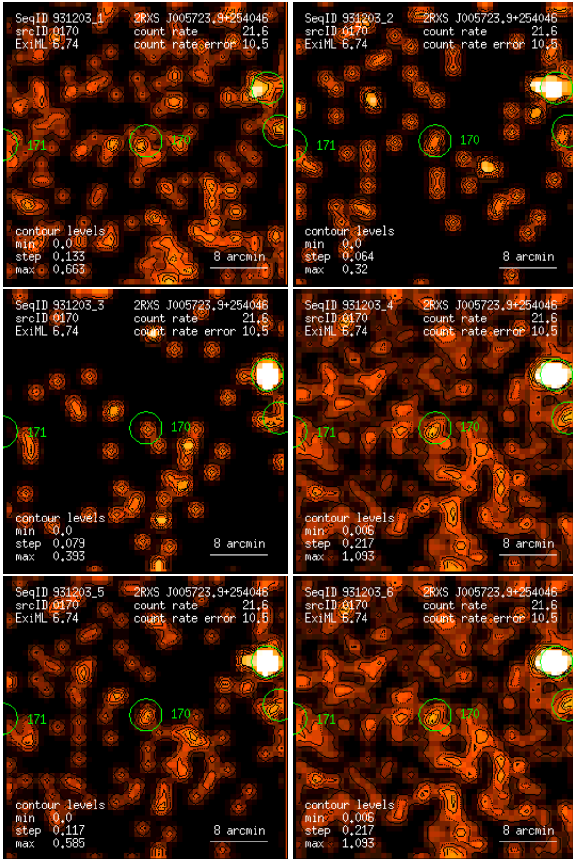
Figure 170: RASS 931203: detection 0170: band rate images, Gaussian filter: (1) PSPC channels 11 – 41, (2) 52 – 90, (3) 91 – 201, (4) 11 – 235, (5) 52 – 201, (6) 11 – 201. Broad band rates in counts/ks. Band rate contour levels in counts/ks/arcmin 2 .
