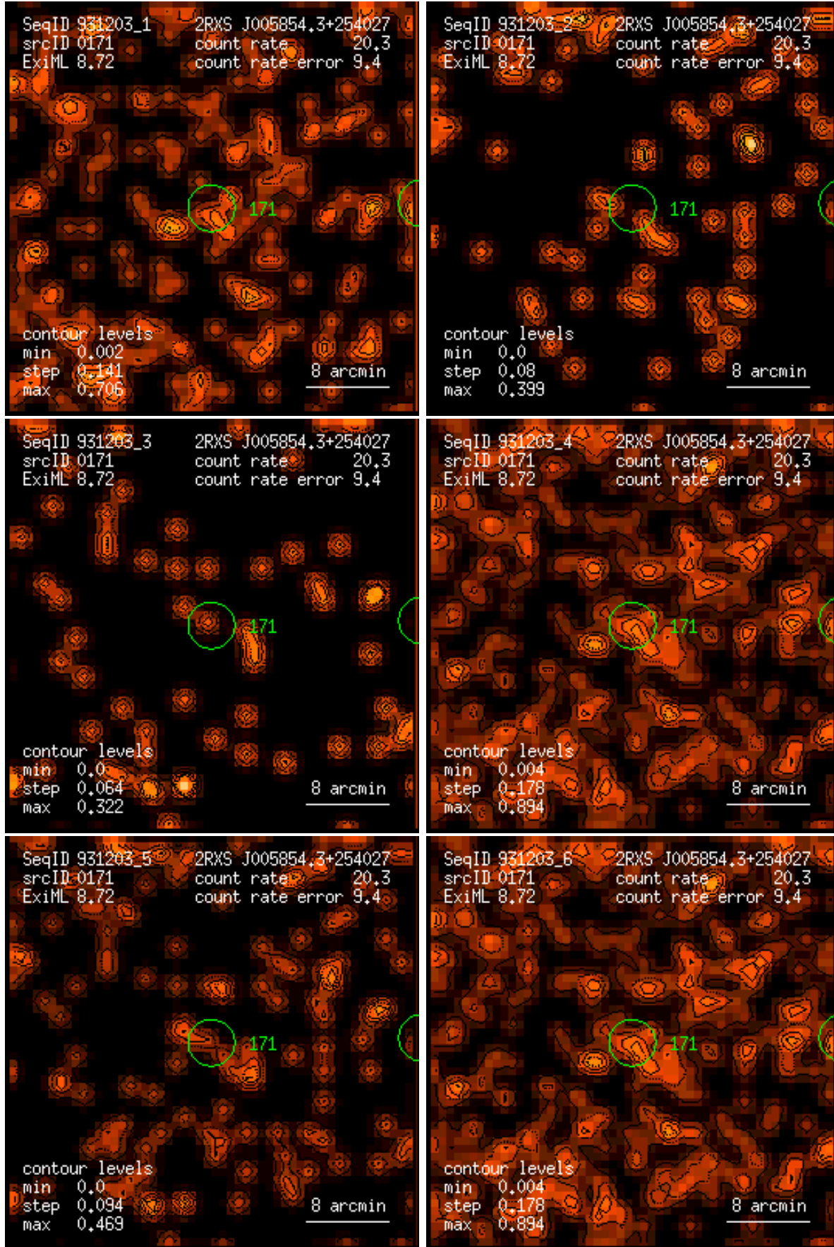
Figure 171: RASS 931203: detection 0171: band rate images, Gaussian filter: (1) PSPC channels 11 – 41, (2) 52 – 90, (3) 91 – 201, (4) 11 – 235, (5) 52 – 201, (6) 11 – 201. Broad band rates in counts/ks. Band rate contour levels in counts/ks/arcmin 2 .
