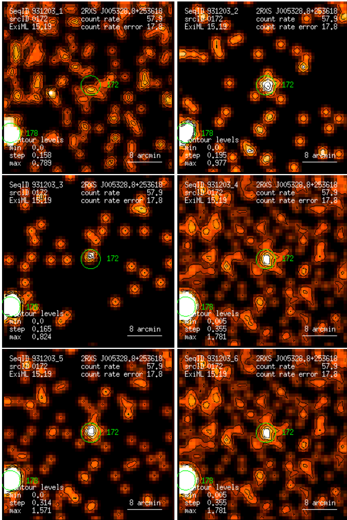
Figure 172: RASS 931203: detection 0172: band rate images, Gaussian filter: (1) PSPC channels 11 – 41, (2) 52 – 90, (3) 91 – 201, (4) 11 – 235, (5) 52 – 201, (6) 11 – 201. Broad band rates in counts/ks. Band rate contour levels in counts/ks/arcmin 2 .
