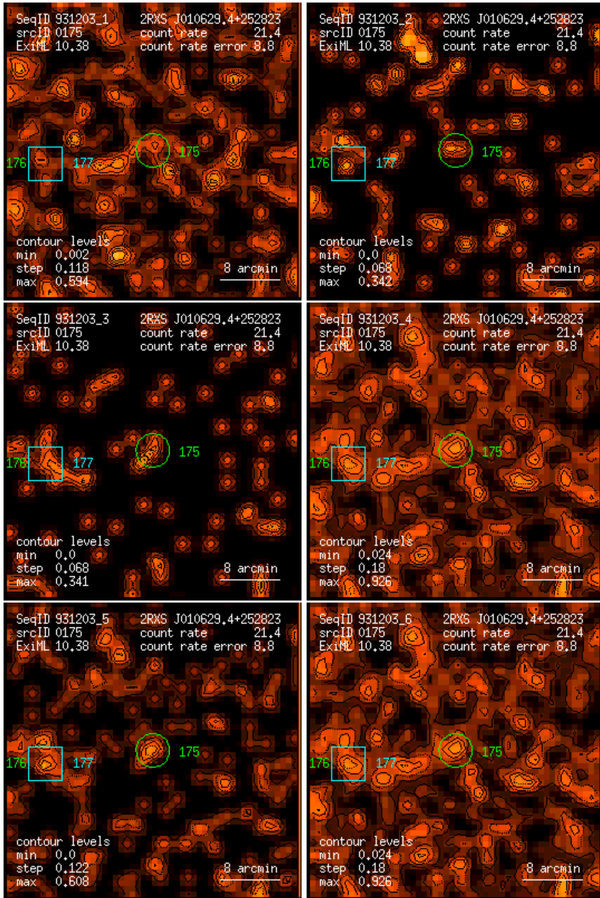
Figure 175: RASS 931203: detection 0175: band rate images, Gaussian filter: (1) PSPC channels 11 – 41, (2) 52 – 90, (3) 91 – 201, (4) 11 – 235, (5) 52 – 201, (6) 11 – 201. Broad band rates in counts/ks. Band rate contour levels in counts/ks/arcmin 2 .
