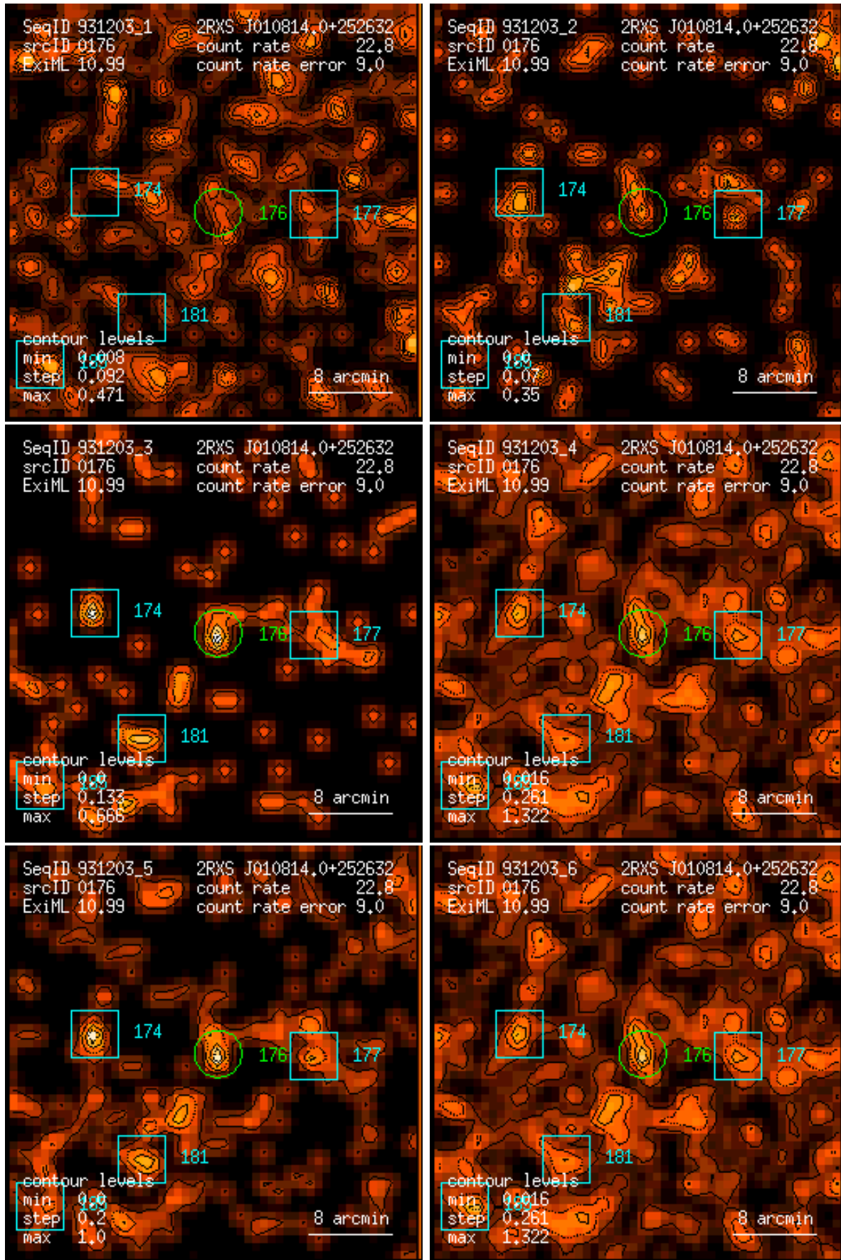
Figure 176: RASS 931203: detection 0176: band rate images, Gaussian filter: (1) PSPC channels 11 – 41, (2) 52 – 90, (3) 91 – 201, (4) 11 – 235, (5) 52 – 201, (6) 11 – 201. Broad band rates in counts/ks. Band rate contour levels in counts/ks/arcmin 2 .
