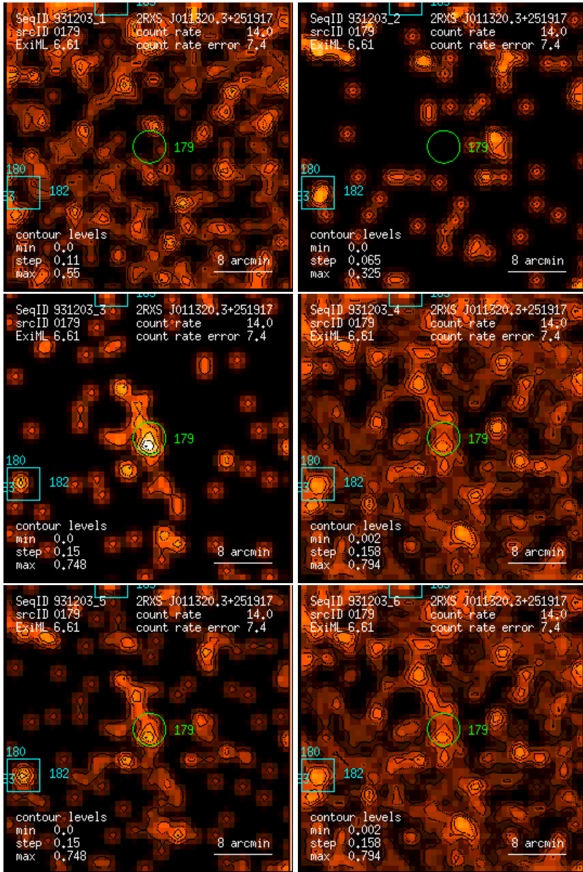
Figure 179: RASS 931203: detection 0179: band rate images, Gaussian filter: (1) PSPC channels 11 – 41, (2) 52 – 90, (3) 91 – 201, (4) 11 – 235, (5) 52 – 201, (6) 11 – 201. Broad band rates in counts/ks. Band rate contour levels in counts/ks/arcmin 2 .
