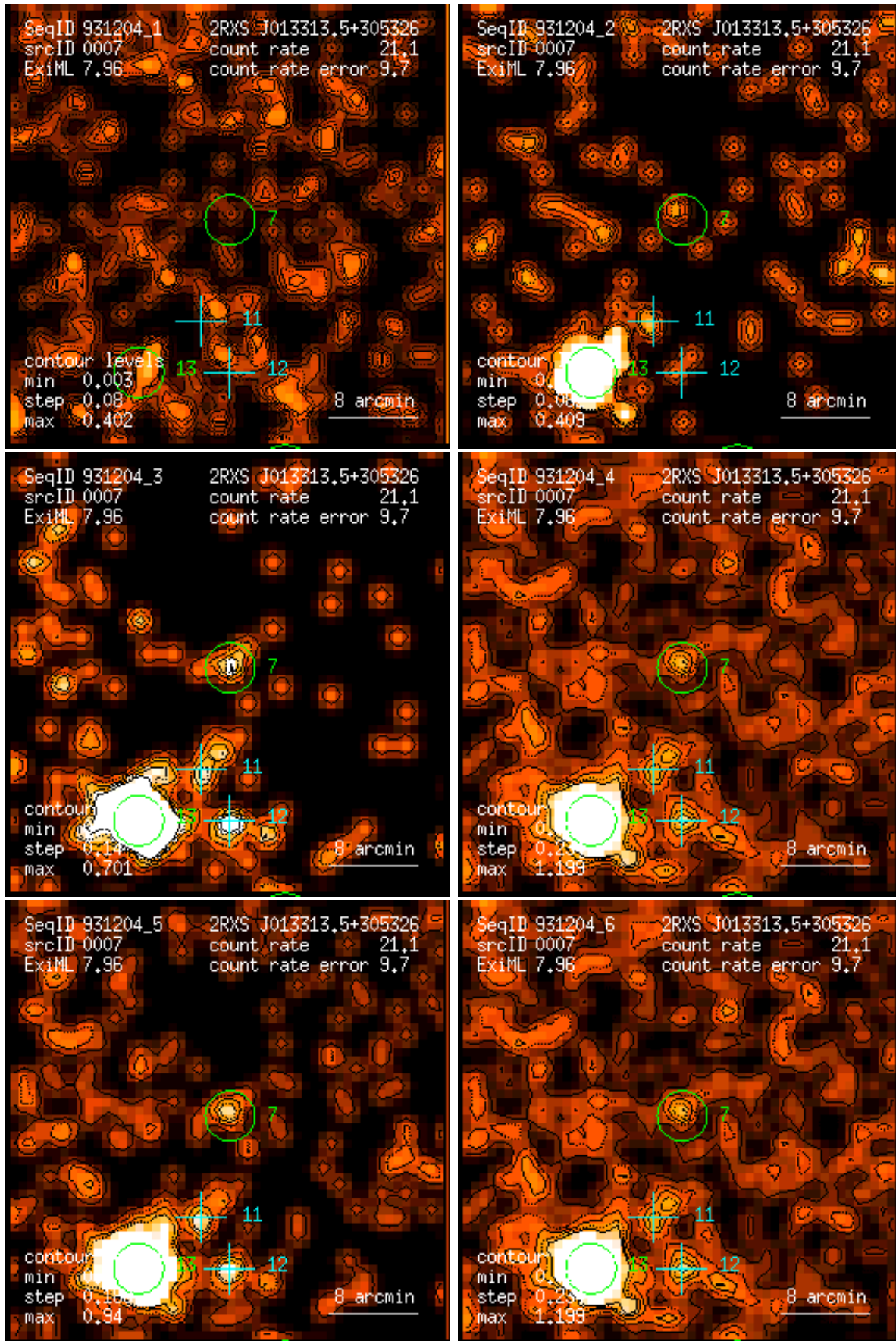
Figure 7: RASS 931204: detection 0007: band rate images, Gaussian filter: (1) PSPC channels 11 – 41, (2) 52 – 90, (3) 91 – 201, (4) 11 – 235, (5) 52 – 201, (6) 11 – 201. Broad band rates in counts/ks. Band rate contour levels in counts/ks/arcmin 2 .
