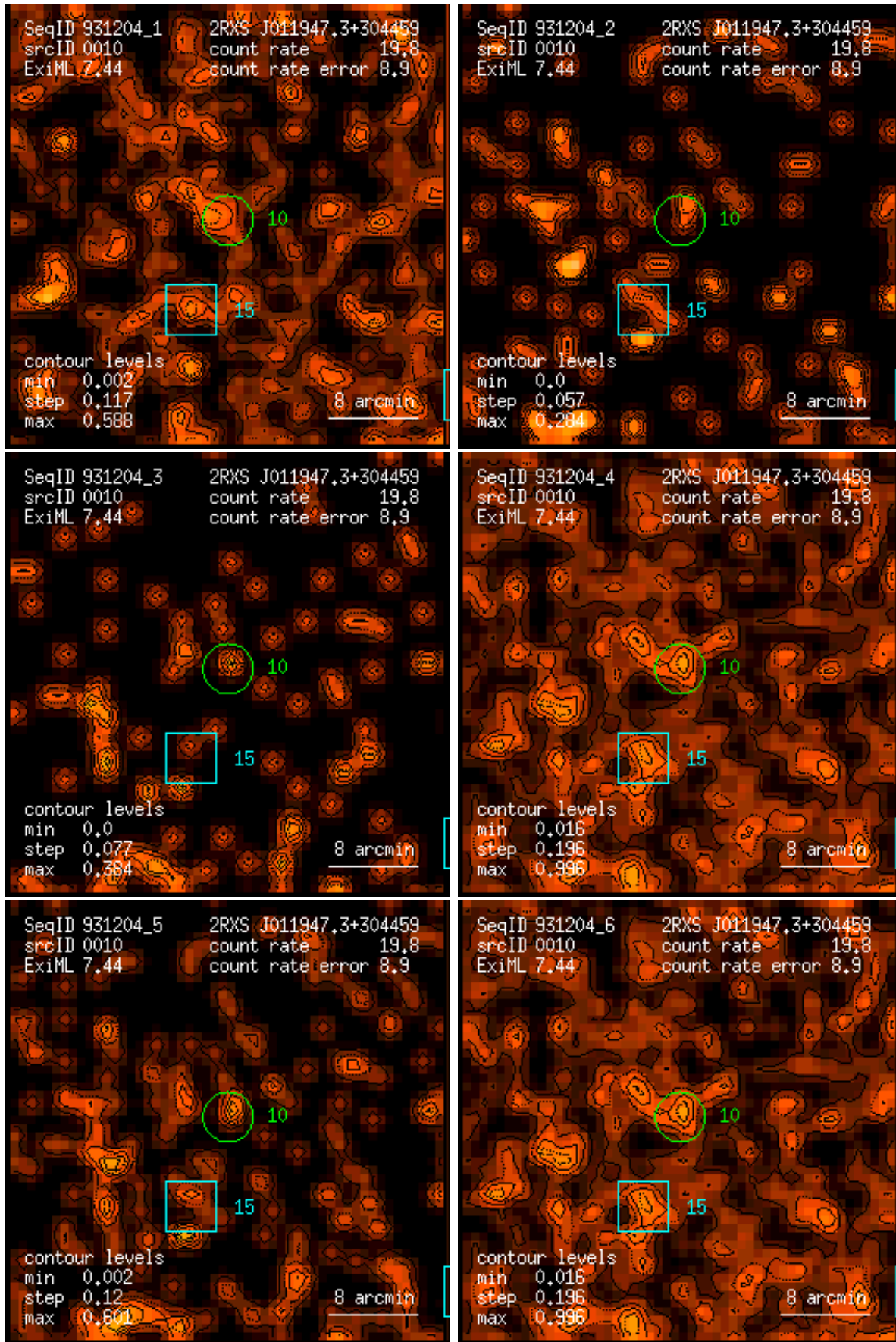
Figure 10: RASS 931204: detection 0010: band rate images, Gaussian filter: (1) PSPC channels 11 – 41, (2) 52 – 90, (3) 91 – 201, (4) 11 – 235, (5) 52 – 201, (6) 11 – 201. Broad band rates in counts/ks. Band rate contour levels in counts/ks/arcmin 2 .
