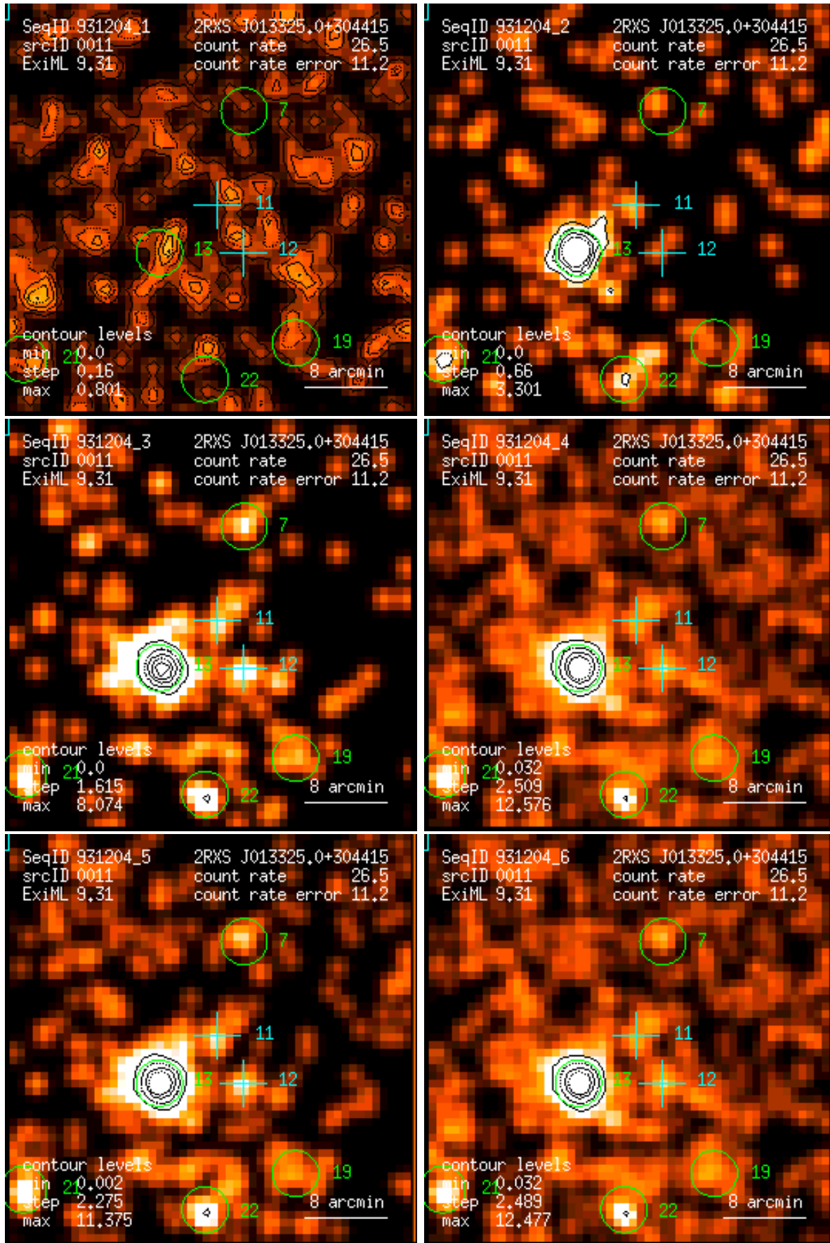
Figure 11: RASS 931204: detection 0011: band rate images, Gaussian filter: (1) PSPC channels 11 – 41, (2) 52 – 90, (3) 91 – 201, (4) 11 – 235, (5) 52 – 201, (6) 11 – 201. Broad band rates in counts/ks. Band rate contour levels in counts/ks/arcmin 2 .
