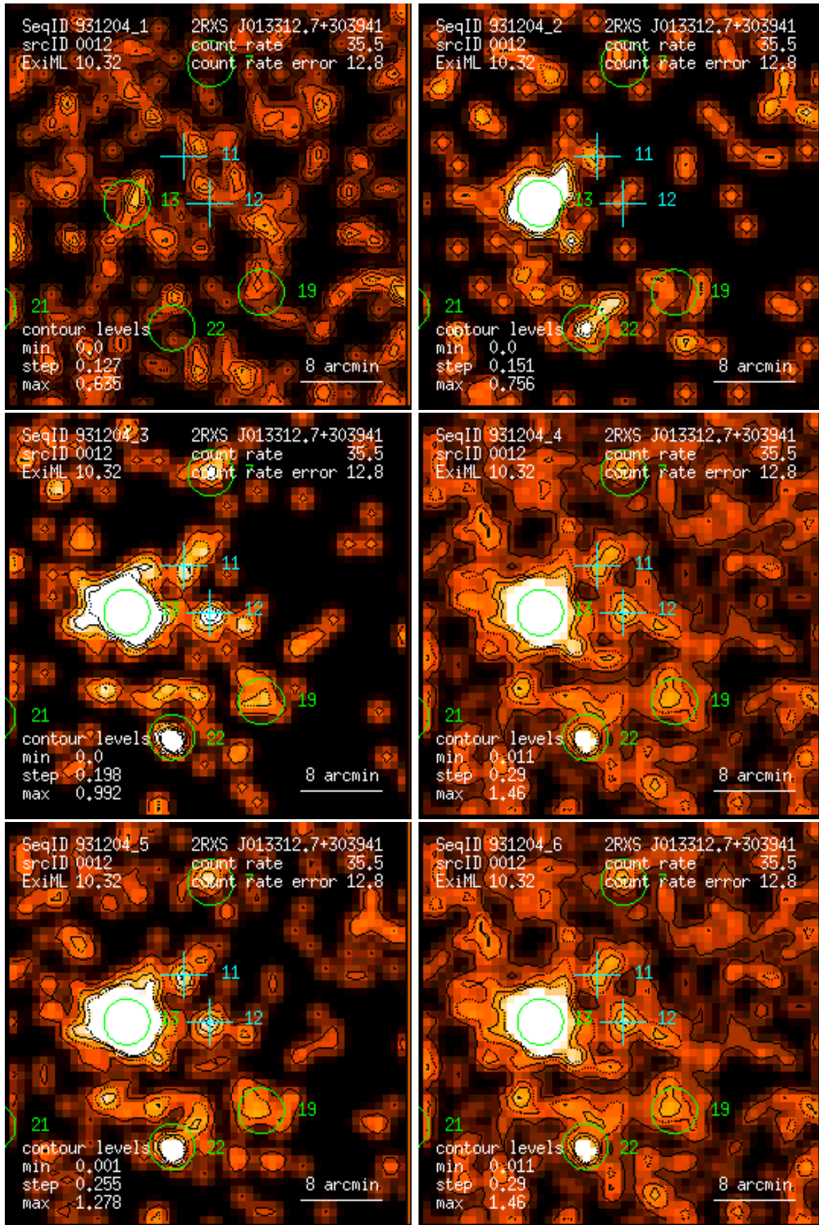
Figure 12: RASS 931204: detection 0012: band rate images, Gaussian filter: (1) PSPC channels 11 – 41, (2) 52 – 90, (3) 91 – 201, (4) 11 – 235, (5) 52 – 201, (6) 11 – 201. Broad band rates in counts/ks. Band rate contour levels in counts/ks/arcmin 2 .
