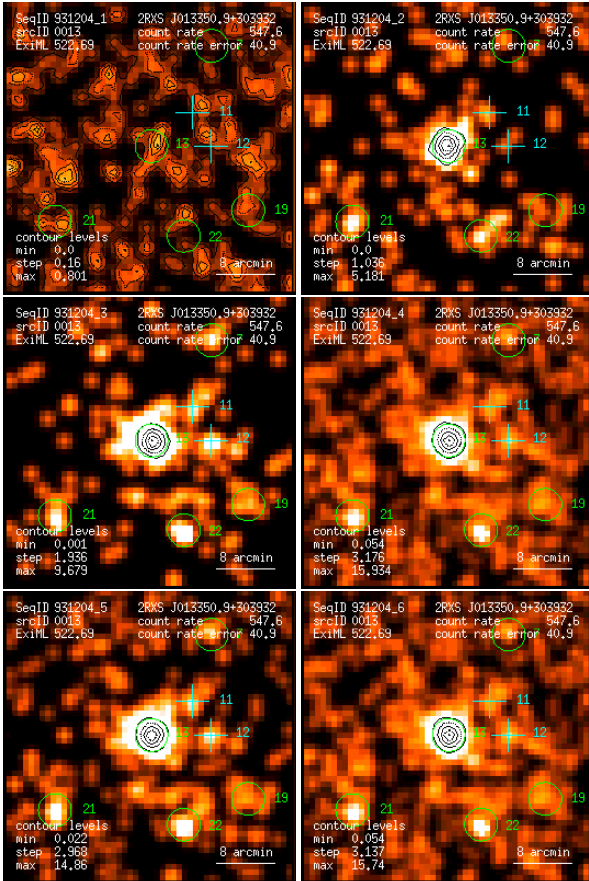
Figure 13: RASS 931204: detection 0013: band rate images, Gaussian filter: (1) PSPC channels 11 – 41, (2) 52 – 90, (3) 91 – 201, (4) 11 – 235, (5) 52 – 201, (6) 11 – 201. Broad band rates in counts/ks. Band rate contour levels in counts/ks/arcmin 2 .
