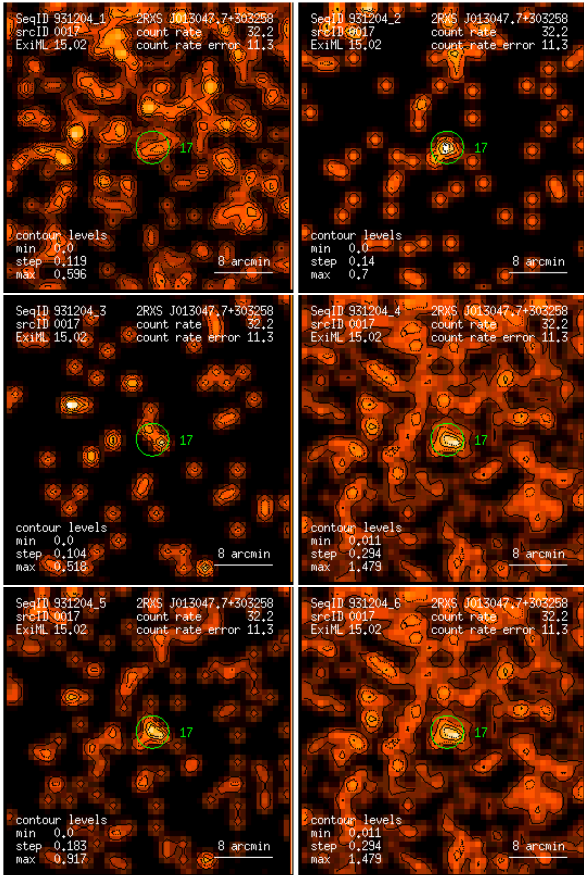
Figure 17: RASS 931204: detection 0017: band rate images, Gaussian filter: (1) PSPC channels 11 – 41, (2) 52 – 90, (3) 91 – 201, (4) 11 – 235, (5) 52 – 201, (6) 11 – 201. Broad band rates in counts/ks. Band rate contour levels in counts/ks/arcmin 2 .
