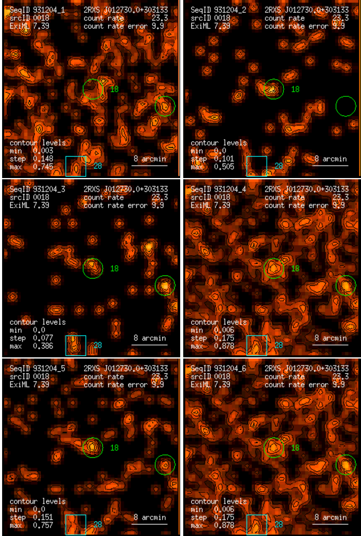
Figure 18: RASS 931204: detection 0018: band rate images, Gaussian filter: (1) PSPC channels 11 – 41, (2) 52 – 90, (3) 91 – 201, (4) 11 – 235, (5) 52 – 201, (6) 11 – 201. Broad band rates in counts/ks. Band rate contour levels in counts/ks/arcmin 2 .
