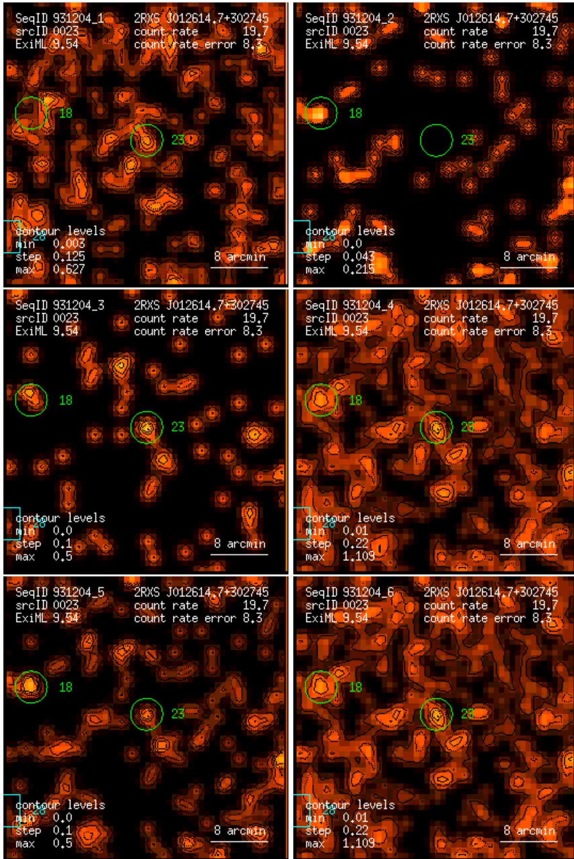
Figure 23: RASS 931204: detection 0023: band rate images, Gaussian filter: (1) PSPC channels 11 – 41, (2) 52 – 90, (3) 91 – 201, (4) 11 – 235, (5) 52 – 201, (6) 11 – 201. Broad band rates in counts/ks. Band rate contour levels in counts/ks/arcmin 2 .
