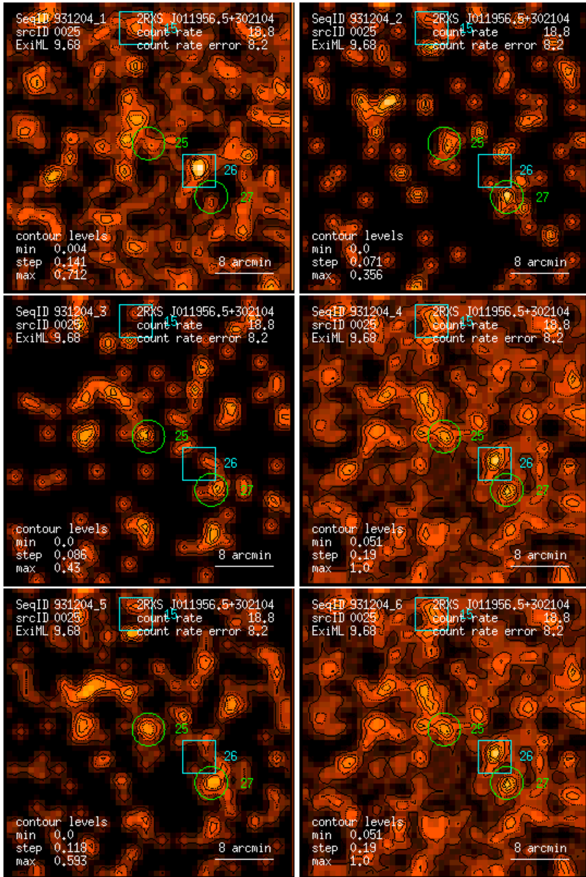
Figure 25: RASS 931204: detection 0025: band rate images, Gaussian filter: (1) PSPC channels 11 – 41, (2) 52 – 90, (3) 91 – 201, (4) 11 – 235, (5) 52 – 201, (6) 11 – 201. Broad band rates in counts/ks. Band rate contour levels in counts/ks/arcmin 2 .
