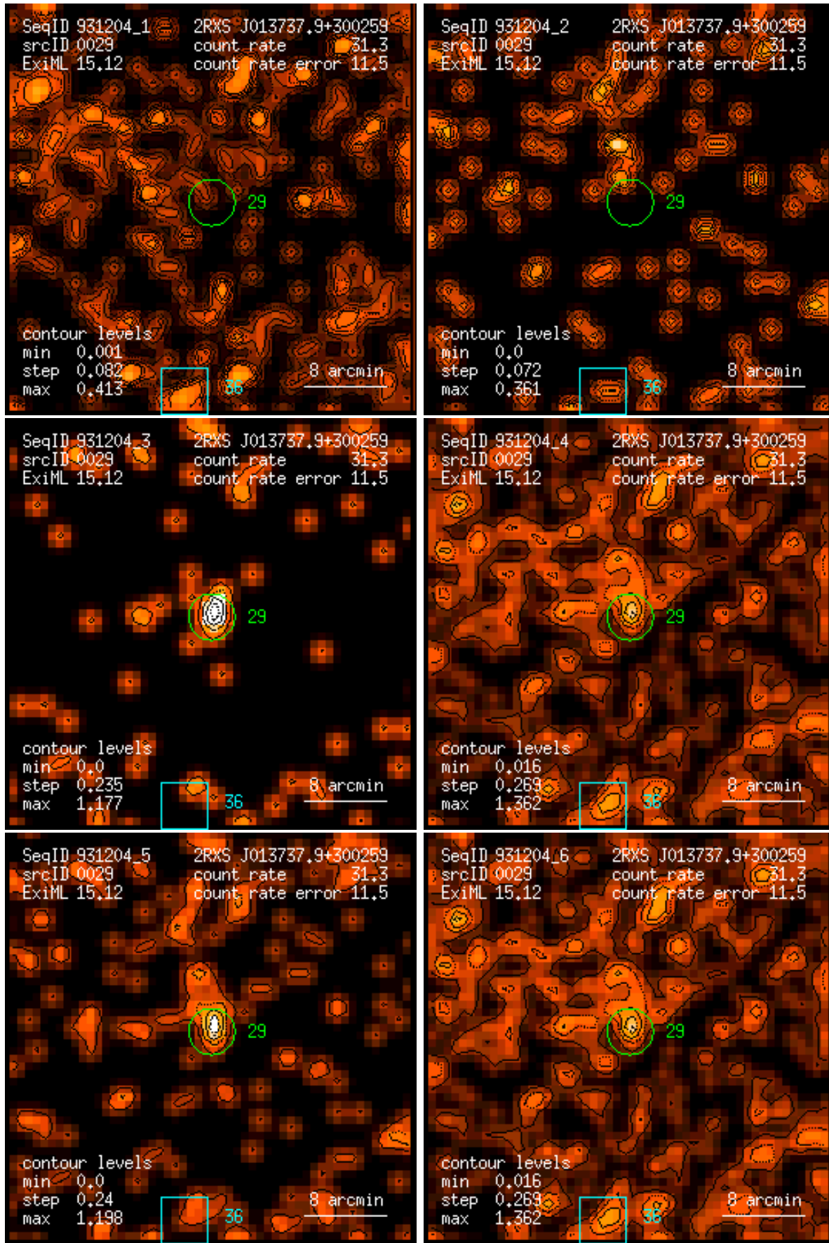
Figure 29: RASS 931204: detection 0029: band rate images, Gaussian filter: (1) PSPC channels 11 – 41, (2) 52 – 90, (3) 91 – 201, (4) 11 – 235, (5) 52 – 201, (6) 11 – 201. Broad band rates in counts/ks. Band rate contour levels in counts/ks/arcmin 2 .
