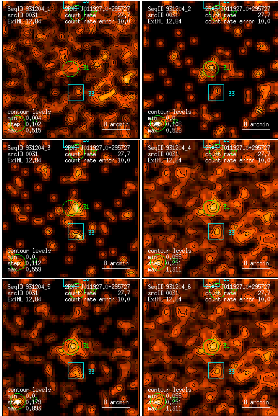
Figure 31: RASS 931204: detection 0031: band rate images, Gaussian filter: (1) PSPC channels 11 – 41, (2) 52 – 90, (3) 91 – 201, (4) 11 – 235, (5) 52 – 201, (6) 11 – 201. Broad band rates in counts/ks. Band rate contour levels in counts/ks/arcmin 2 .
