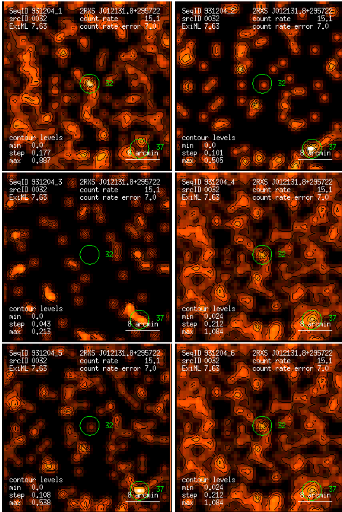
Figure 32: RASS 931204: detection 0032: band rate images, Gaussian filter: (1) PSPC channels 11 – 41, (2) 52 – 90, (3) 91 – 201, (4) 11 – 235, (5) 52 – 201, (6) 11 – 201. Broad band rates in counts/ks. Band rate contour levels in counts/ks/arcmin 2 .
