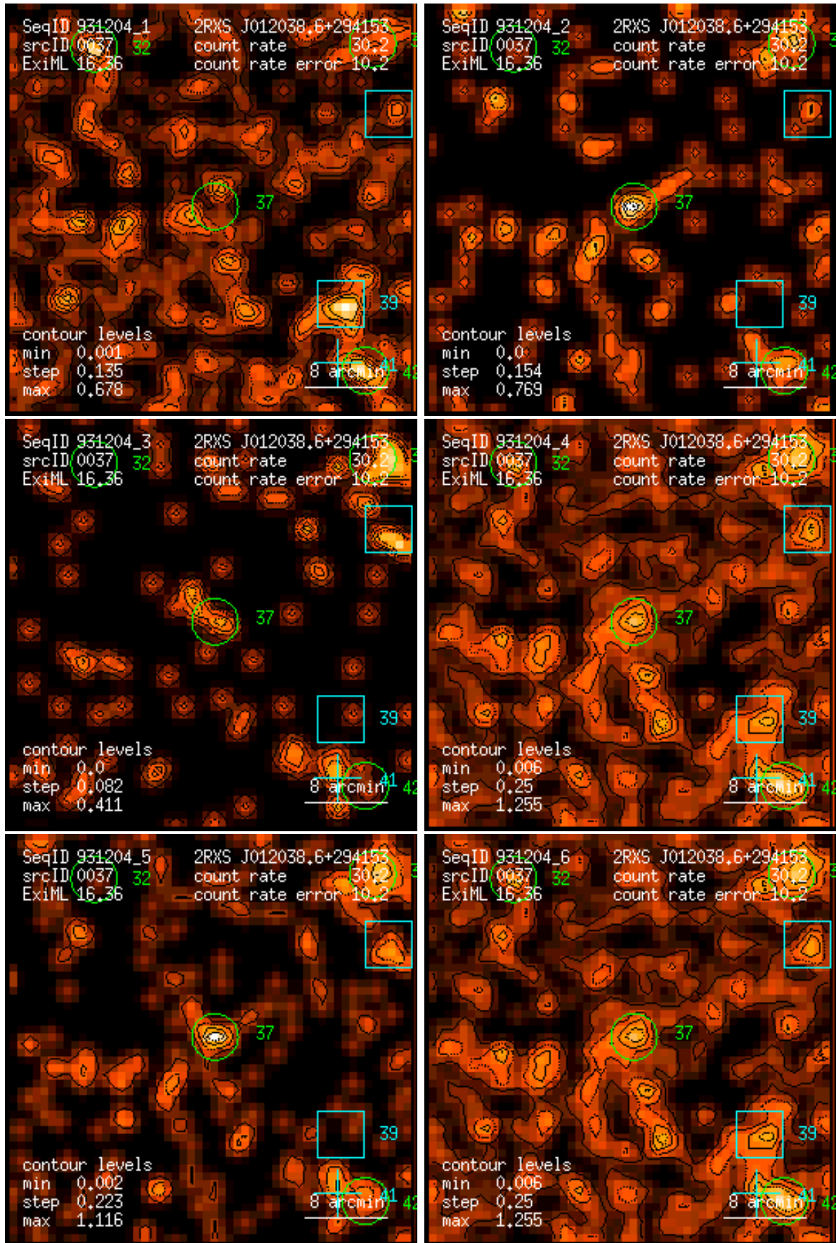
Figure 37: RASS 931204: detection 0037: band rate images, Gaussian filter: (1) PSPC channels 11 – 41, (2) 52 – 90, (3) 91 – 201, (4) 11 – 235, (5) 52 – 201, (6) 11 – 201. Broad band rates in counts/ks. Band rate contour levels in counts/ks/arcmin 2 .
