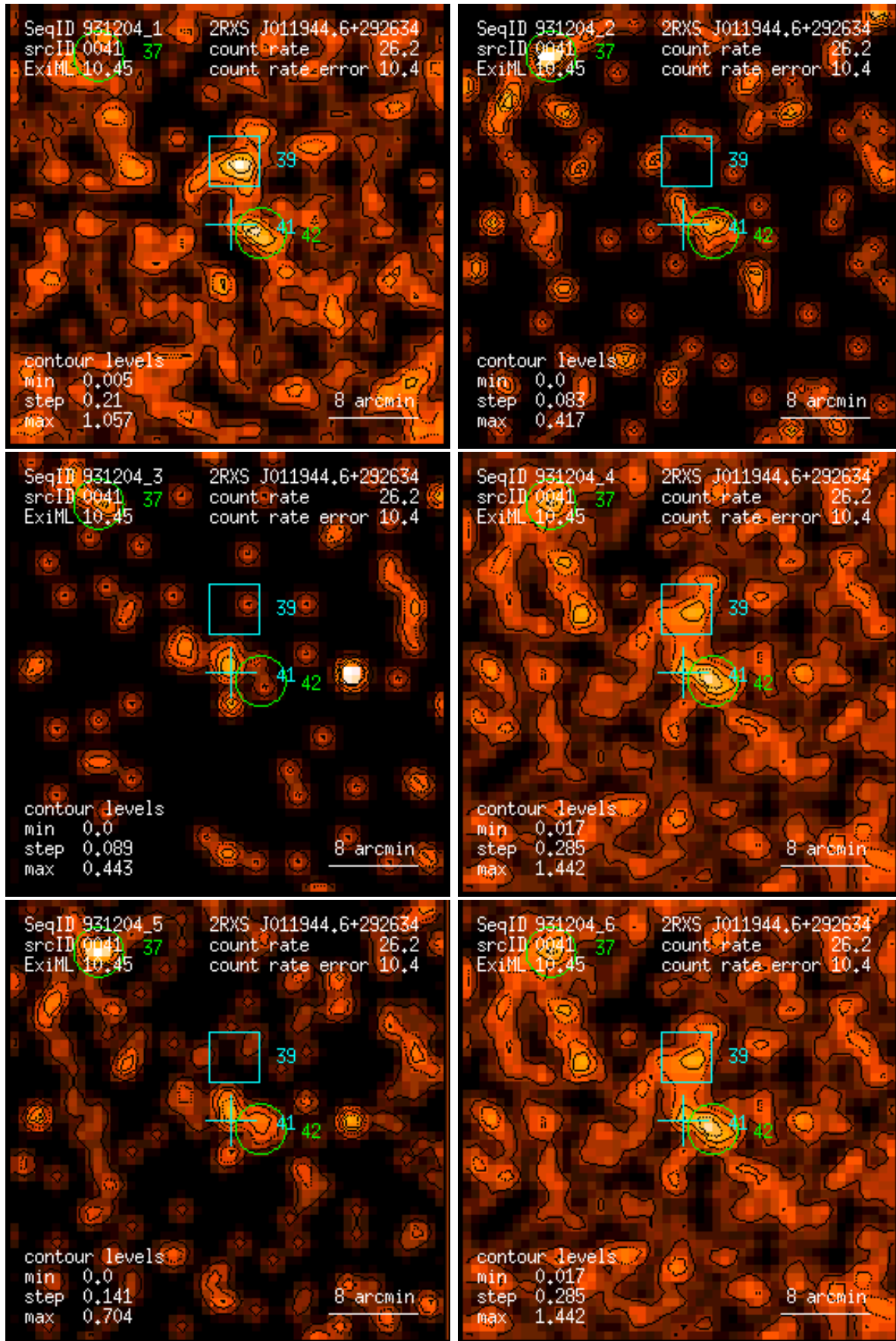
Figure 41: RASS 931204: detection 0041: band rate images, Gaussian filter: (1) PSPC channels 11 – 41, (2) 52 – 90, (3) 91 – 201, (4) 11 – 235, (5) 52 – 201, (6) 11 – 201. Broad band rates in counts/ks. Band rate contour levels in counts/ks/arcmin 2 .
