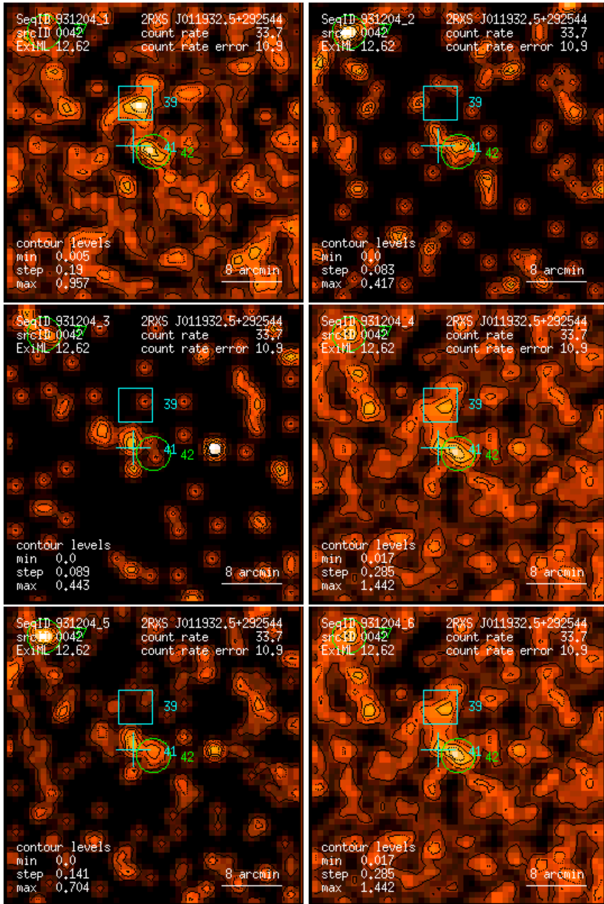
Figure 42: RASS 931204: detection 0042: band rate images, Gaussian filter: (1) PSPC channels 11 – 41, (2) 52 – 90, (3) 91 – 201, (4) 11 – 235, (5) 52 – 201, (6) 11 – 201. Broad band rates in counts/ks. Band rate contour levels in counts/ks/arcmin 2 .
