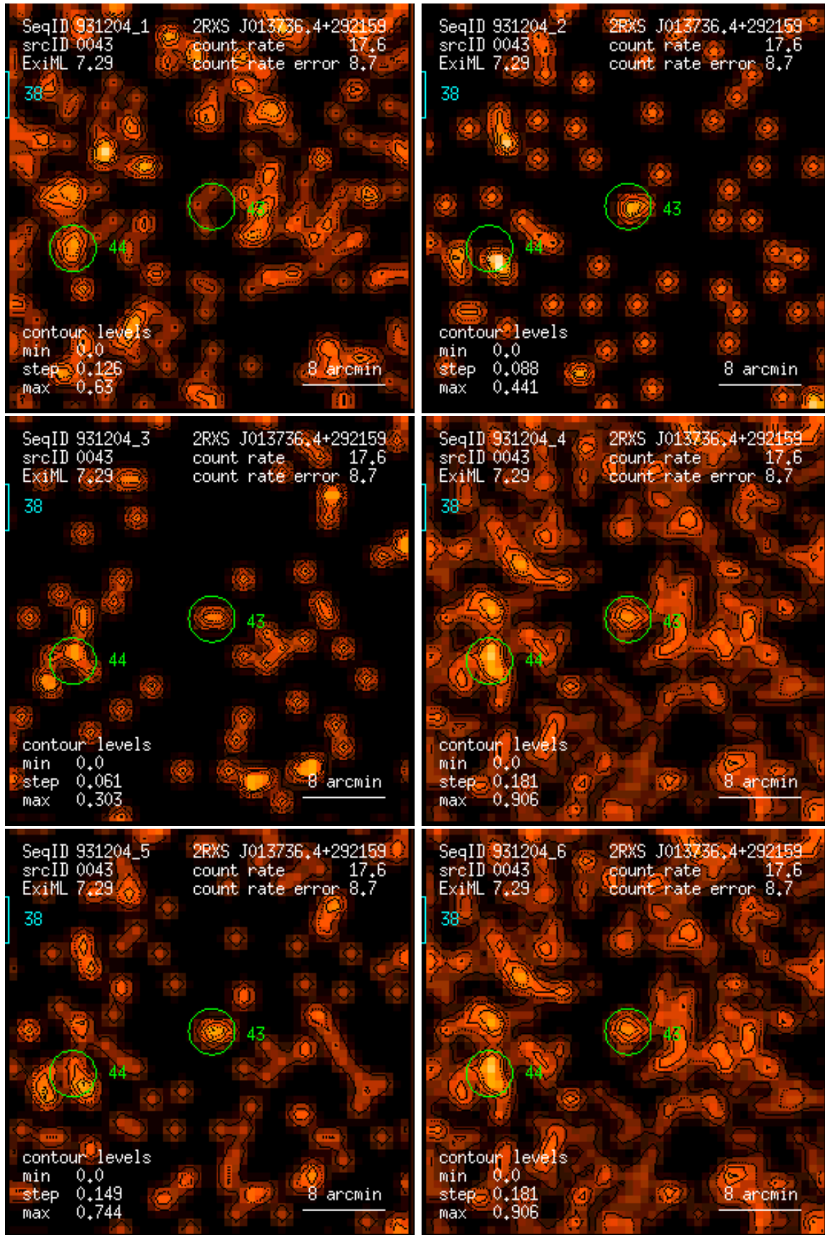
Figure 43: RASS 931204: detection 0043: band rate images, Gaussian filter: (1) PSPC channels 11 – 41, (2) 52 – 90, (3) 91 – 201, (4) 11 – 235, (5) 52 – 201, (6) 11 – 201. Broad band rates in counts/ks. Band rate contour levels in counts/ks/arcmin 2 .
