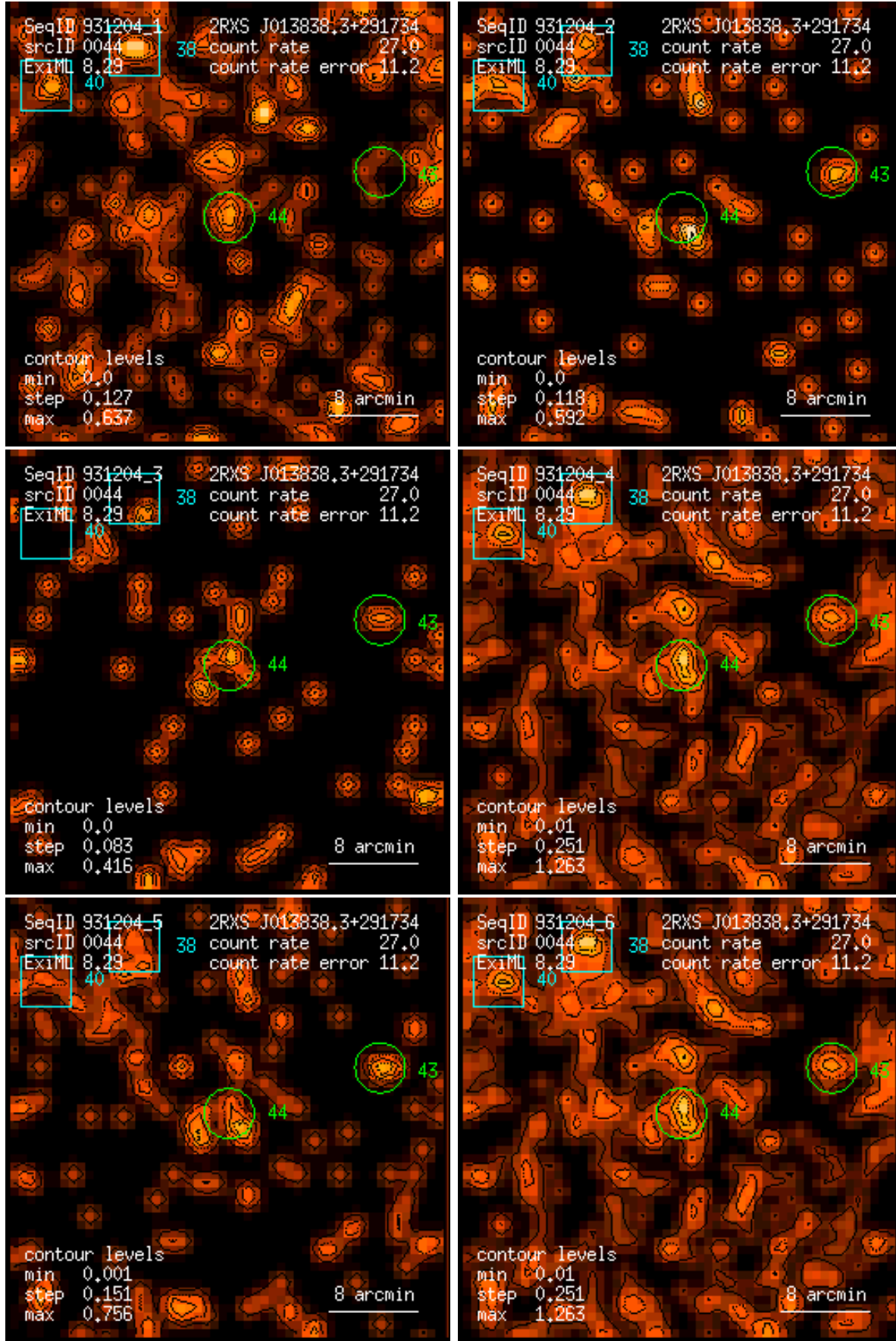
Figure 44: RASS 931204: detection 0044: band rate images, Gaussian filter: (1) PSPC channels 11 – 41, (2) 52 – 90, (3) 91 – 201, (4) 11 – 235, (5) 52 – 201, (6) 11 – 201. Broad band rates in counts/ks. Band rate contour levels in counts/ks/arcmin 2 .
