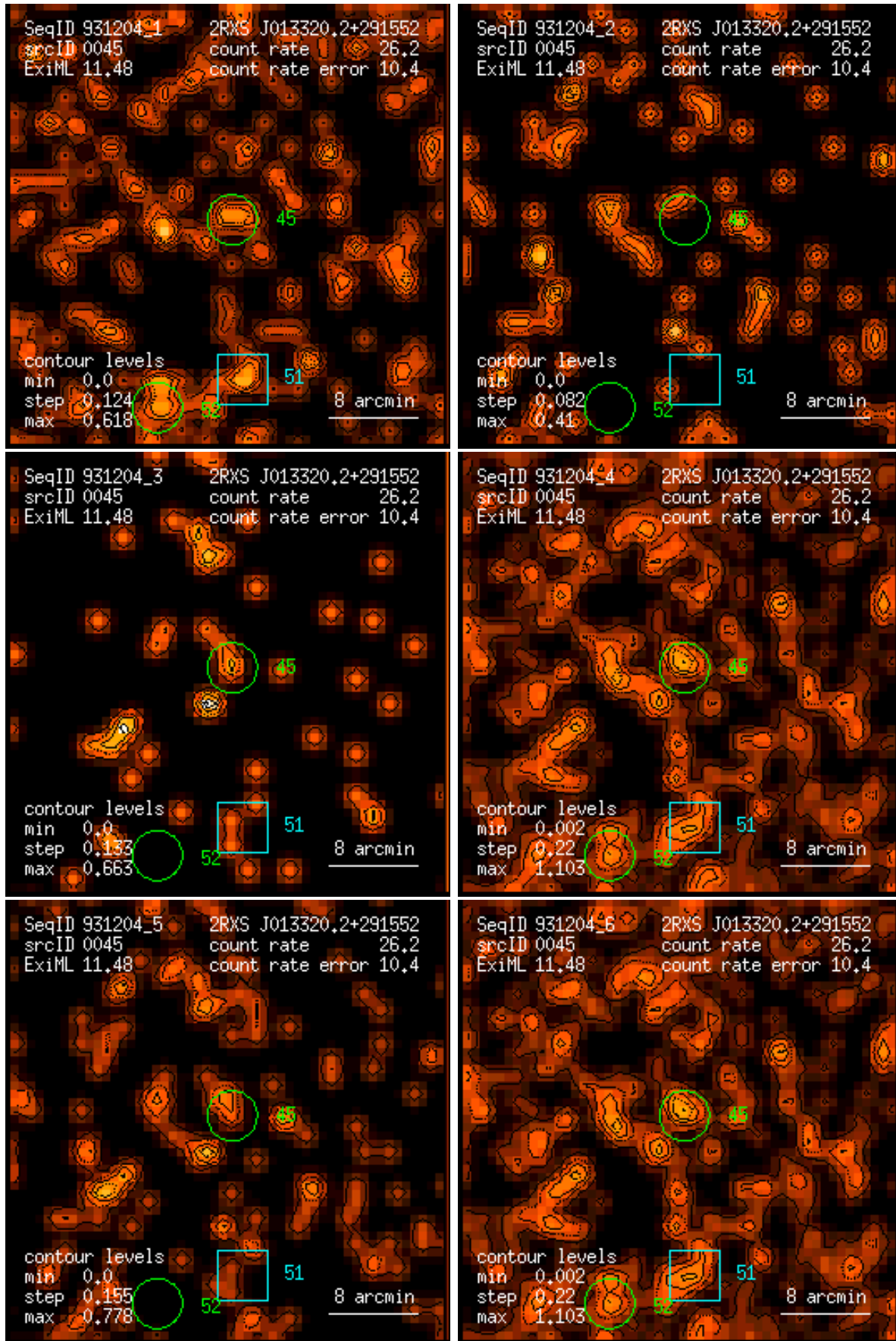
Figure 45: RASS 931204: detection 0045: band rate images, Gaussian filter: (1) PSPC channels 11 – 41, (2) 52 – 90, (3) 91 – 201, (4) 11 – 235, (5) 52 – 201, (6) 11 – 201. Broad band rates in counts/ks. Band rate contour levels in counts/ks/arcmin 2 .
