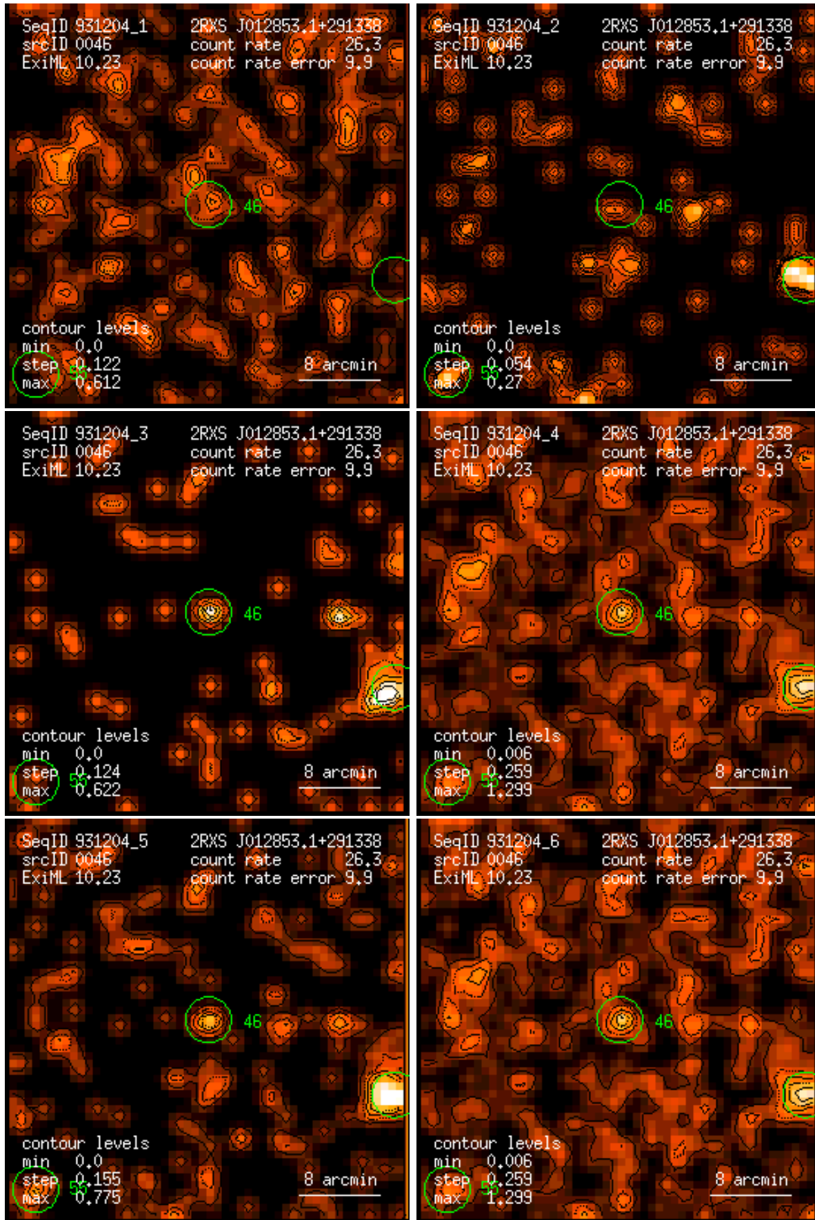
Figure 46: RASS 931204: detection 0046: band rate images, Gaussian filter: (1) PSPC channels 11 – 41, (2) 52 – 90, (3) 91 – 201, (4) 11 – 235, (5) 52 – 201, (6) 11 – 201. Broad band rates in counts/ks. Band rate contour levels in counts/ks/arcmin 2 .
