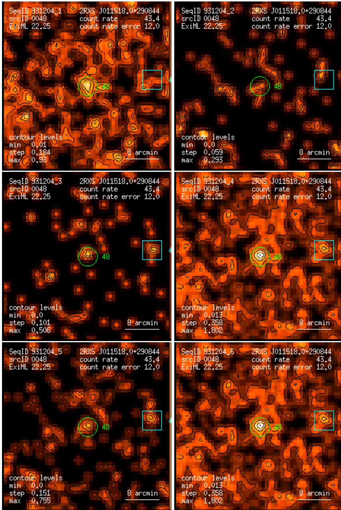
Figure 48: RASS 931204: detection 0048: band rate images, Gaussian filter: (1) PSPC channels 11 – 41, (2) 52 – 90, (3) 91 – 201, (4) 11 – 235, (5) 52 – 201, (6) 11 – 201. Broad band rates in counts/ks. Band rate contour levels in counts/ks/arcmin 2 .
