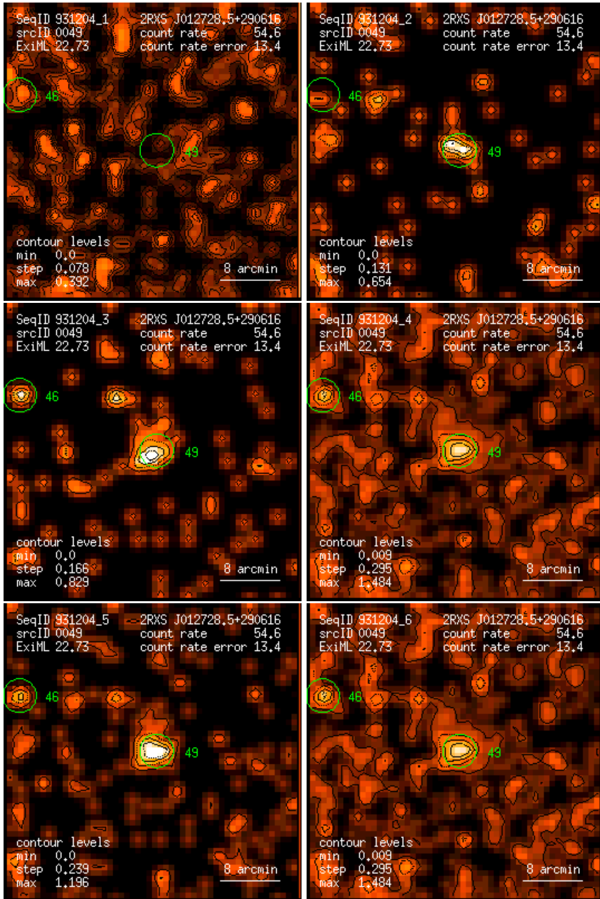
Figure 49: RASS 931204: detection 0049: band rate images, Gaussian filter: (1) PSPC channels 11 – 41, (2) 52 – 90, (3) 91 – 201, (4) 11 – 235, (5) 52 – 201, (6) 11 – 201. Broad band rates in counts/ks. Band rate contour levels in counts/ks/arcmin 2 .
