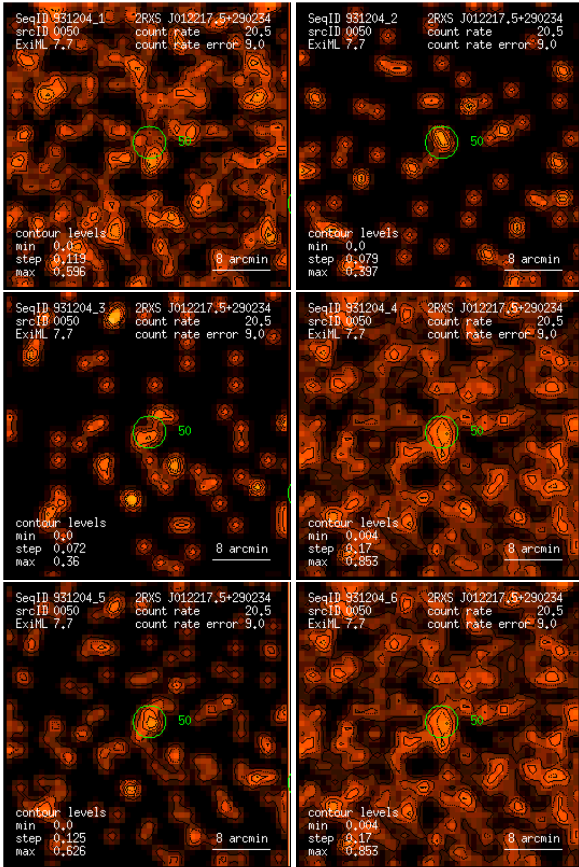
Figure 50: RASS 931204: detection 0050: band rate images, Gaussian filter: (1) PSPC channels 11 – 41, (2) 52 – 90, (3) 91 – 201, (4) 11 – 235, (5) 52 – 201, (6) 11 – 201. Broad band rates in counts/ks. Band rate contour levels in counts/ks/arcmin 2 .
