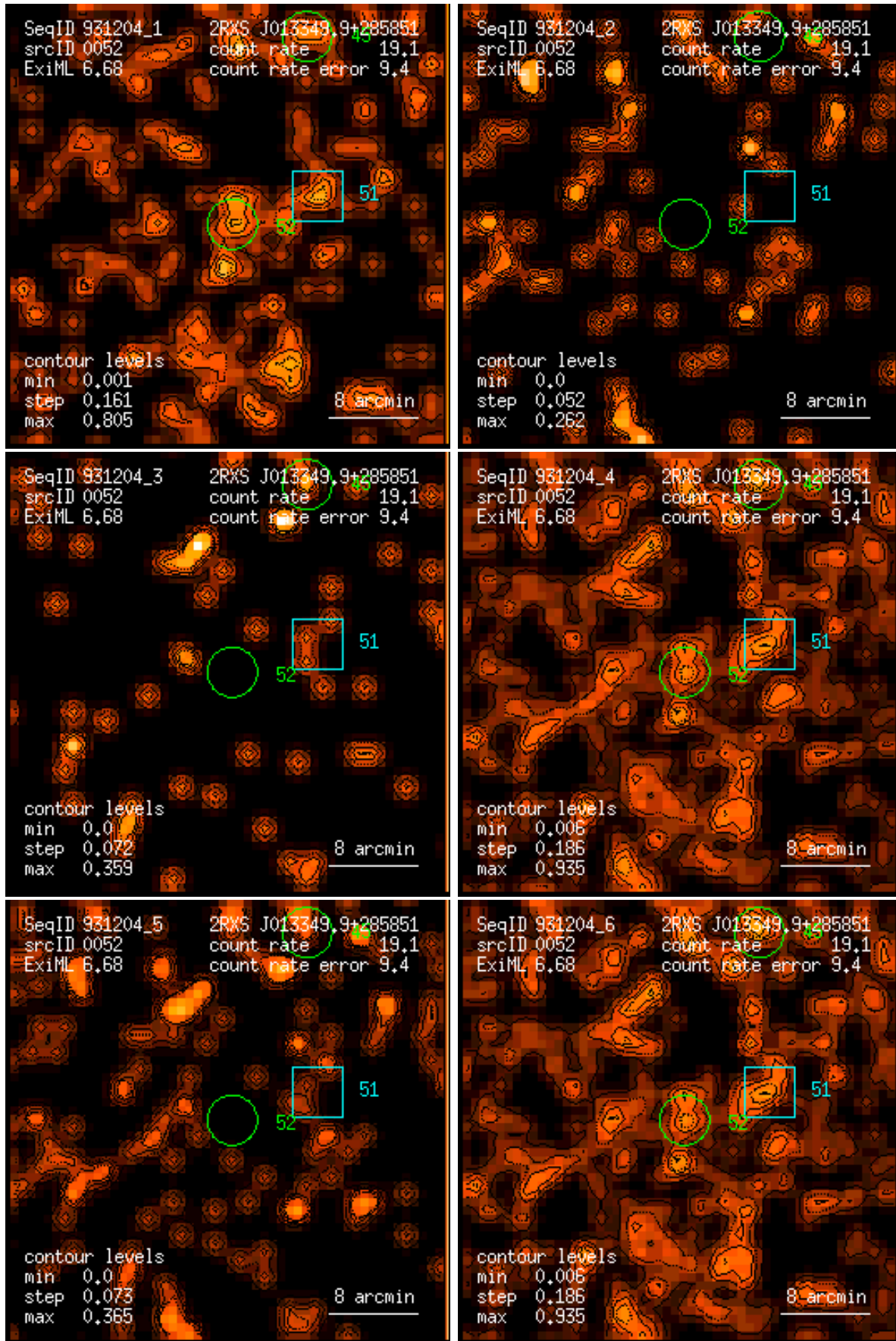
Figure 52: RASS 931204: detection 0052: band rate images, Gaussian filter: (1) PSPC channels 11 – 41, (2) 52 – 90, (3) 91 – 201, (4) 11 – 235, (5) 52 – 201, (6) 11 – 201. Broad band rates in counts/ks. Band rate contour levels in counts/ks/arcmin 2 .
