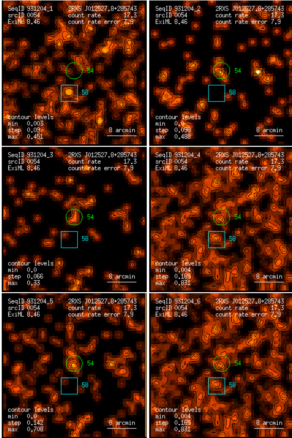
Figure 54: RASS 931204: detection 0054: band rate images, Gaussian filter: (1) PSPC channels 11 – 41, (2) 52 – 90, (3) 91 – 201, (4) 11 – 235, (5) 52 – 201, (6) 11 – 201. Broad band rates in counts/ks. Band rate contour levels in counts/ks/arcmin 2 .
