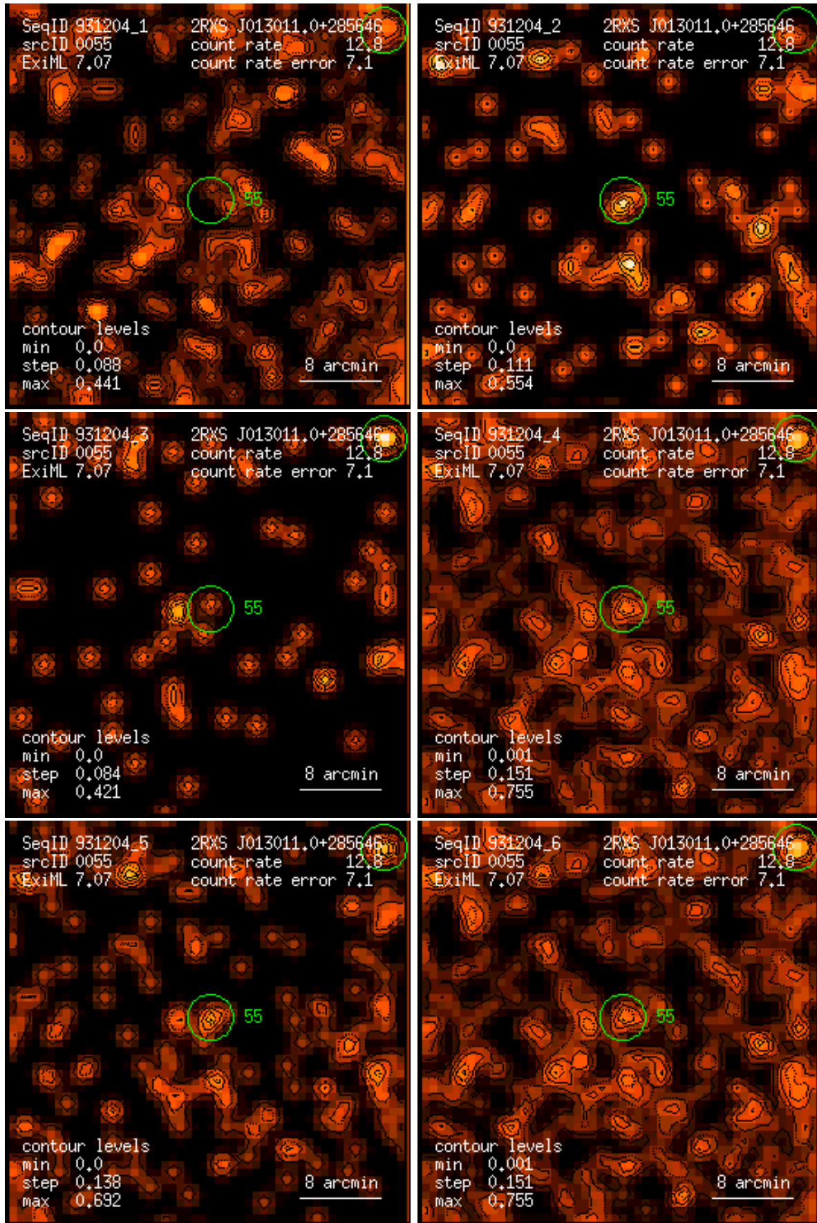
Figure 55: RASS 931204: detection 0055: band rate images, Gaussian filter: (1) PSPC channels 11 – 41, (2) 52 – 90, (3) 91 – 201, (4) 11 – 235, (5) 52 – 201, (6) 11 – 201. Broad band rates in counts/ks. Band rate contour levels in counts/ks/arcmin 2 .
