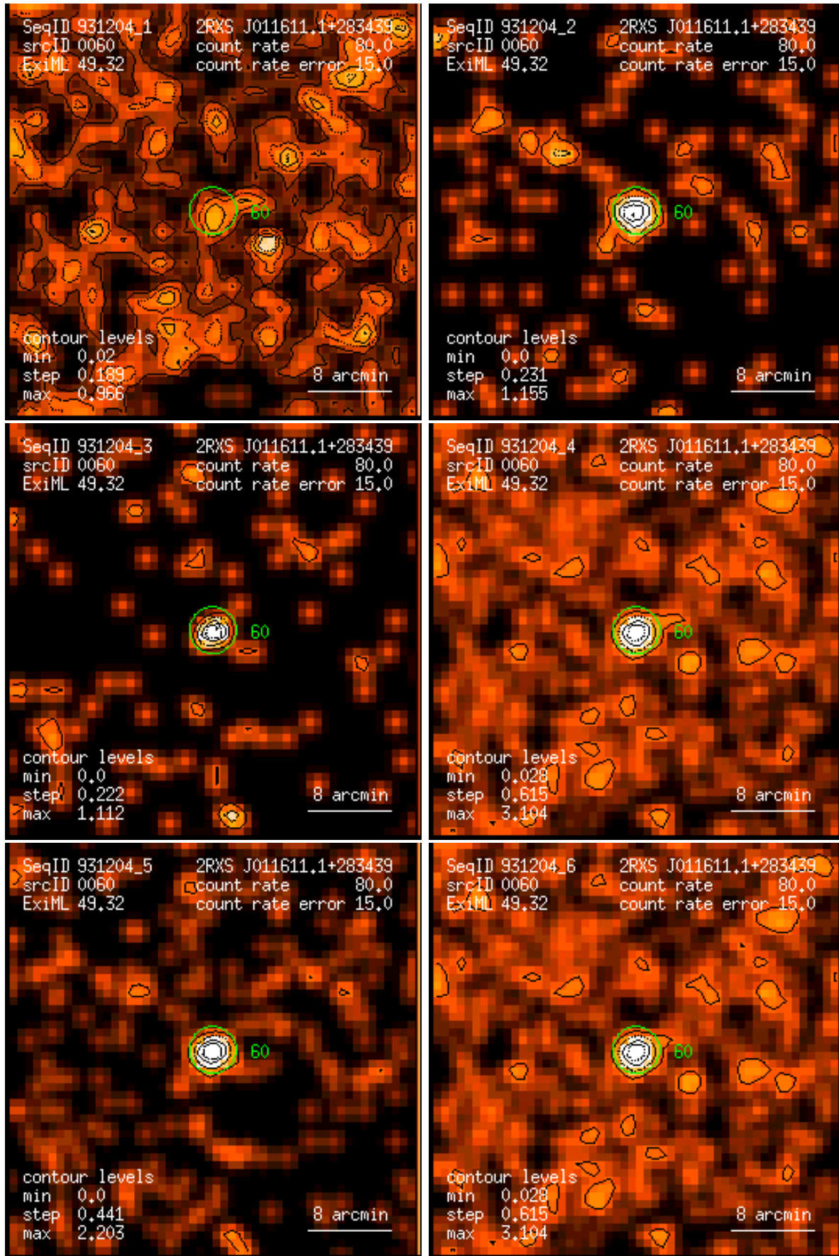
Figure 60: RASS 931204: detection 0060: band rate images, Gaussian filter: (1) PSPC channels 11 – 41, (2) 52 – 90, (3) 91 – 201, (4) 11 – 235, (5) 52 – 201, (6) 11 – 201. Broad band rates in counts/ks. Band rate contour levels in counts/ks/arcmin 2 .
