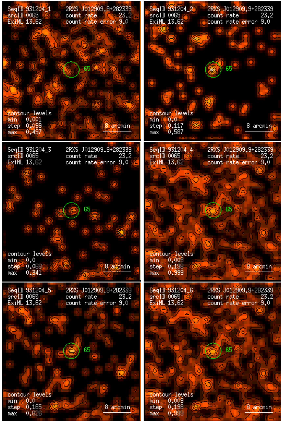
Figure 65: RASS 931204: detection 0065: band rate images, Gaussian filter: (1) PSPC channels 11 – 41, (2) 52 – 90, (3) 91 – 201, (4) 11 – 235, (5) 52 – 201, (6) 11 – 201. Broad band rates in counts/ks. Band rate contour levels in counts/ks/arcmin 2 .
