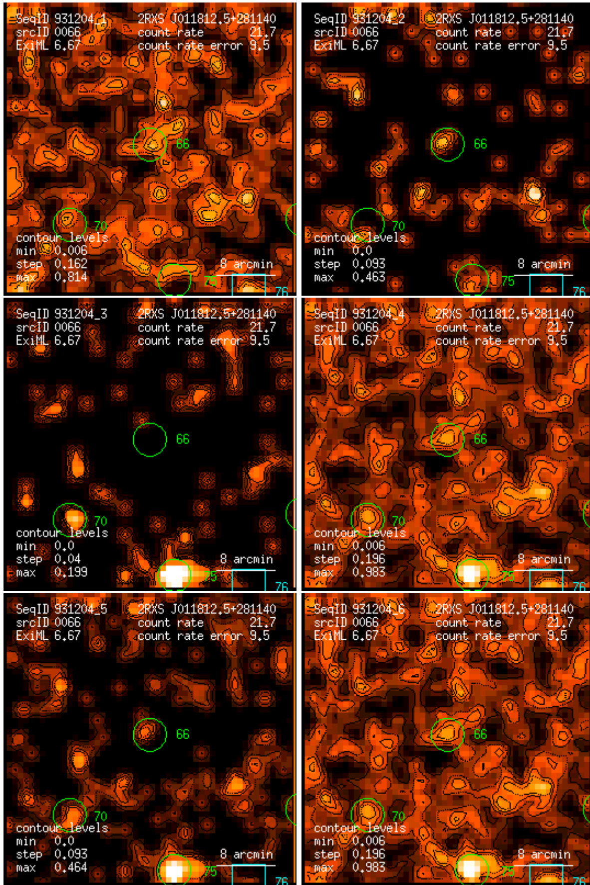
Figure 66: RASS 931204: detection 0066: band rate images, Gaussian filter: (1) PSPC channels 11 – 41, (2) 52 – 90, (3) 91 – 201, (4) 11 – 235, (5) 52 – 201, (6) 11 – 201. Broad band rates in counts/ks. Band rate contour levels in counts/ks/arcmin 2 .
