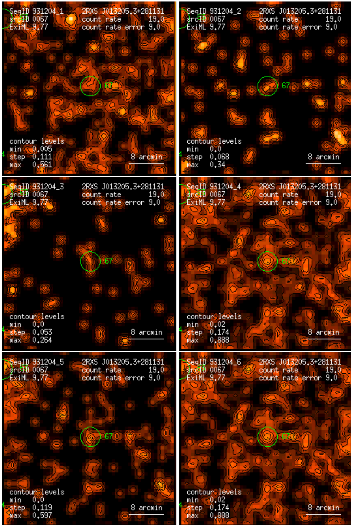
Figure 67: RASS 931204: detection 0067: band rate images, Gaussian filter: (1) PSPC channels 11 – 41, (2) 52 – 90, (3) 91 – 201, (4) 11 – 235, (5) 52 – 201, (6) 11 – 201. Broad band rates in counts/ks. Band rate contour levels in counts/ks/arcmin 2 .
