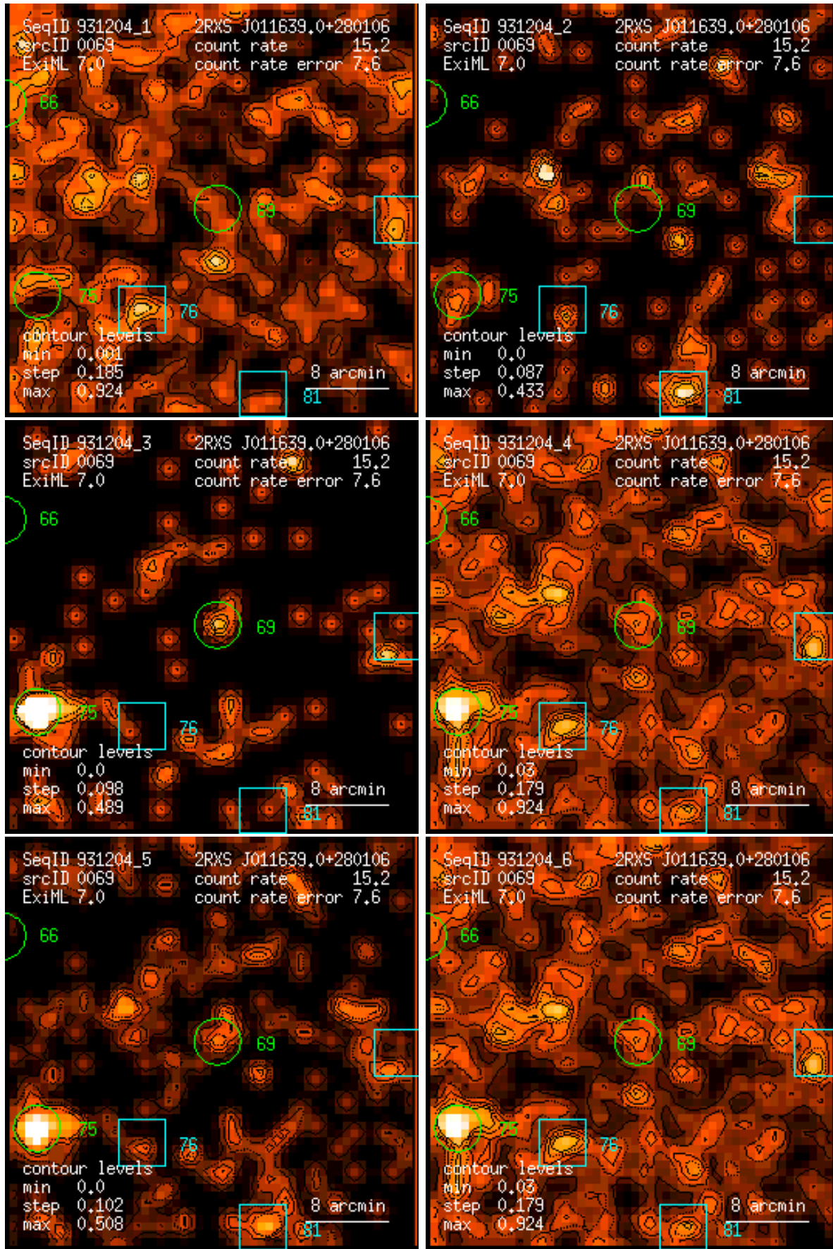
Figure 69: RASS 931204: detection 0069: band rate images, Gaussian filter: (1) PSPC channels 11 – 41, (2) 52 – 90, (3) 91 – 201, (4) 11 – 235, (5) 52 – 201, (6) 11 – 201. Broad band rates in counts/ks. Band rate contour levels in counts/ks/arcmin 2 .
