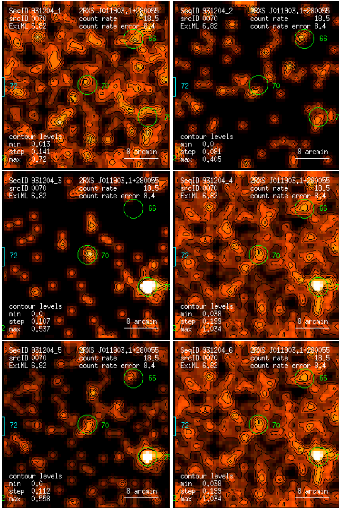
Figure 70: RASS 931204: detection 0070: band rate images, Gaussian filter: (1) PSPC channels 11 – 41, (2) 52 – 90, (3) 91 – 201, (4) 11 – 235, (5) 52 – 201, (6) 11 – 201. Broad band rates in counts/ks. Band rate contour levels in counts/ks/arcmin 2 .
