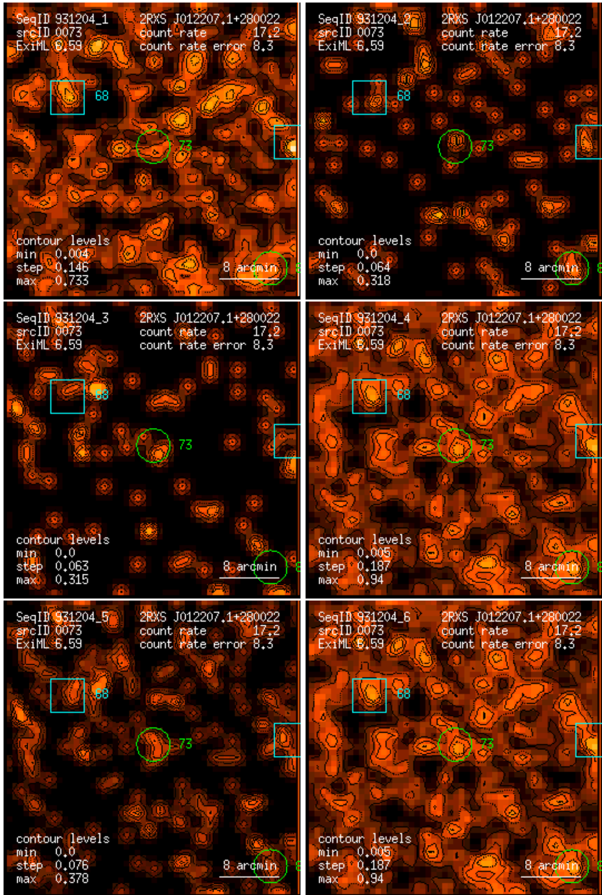
Figure 73: RASS 931204: detection 0073: band rate images, Gaussian filter: (1) PSPC channels 11 – 41, (2) 52 – 90, (3) 91 – 201, (4) 11 – 235, (5) 52 – 201, (6) 11 – 201. Broad band rates in counts/ks. Band rate contour levels in counts/ks/arcmin 2 .
