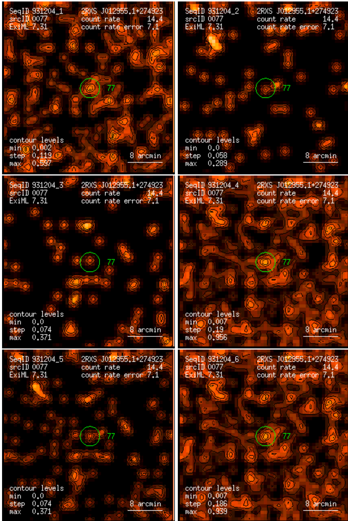
Figure 77: RASS 931204: detection 0077: band rate images, Gaussian filter: (1) PSPC channels 11 – 41, (2) 52 – 90, (3) 91 – 201, (4) 11 – 235, (5) 52 – 201, (6) 11 – 201. Broad band rates in counts/ks. Band rate contour levels in counts/ks/arcmin 2 .
