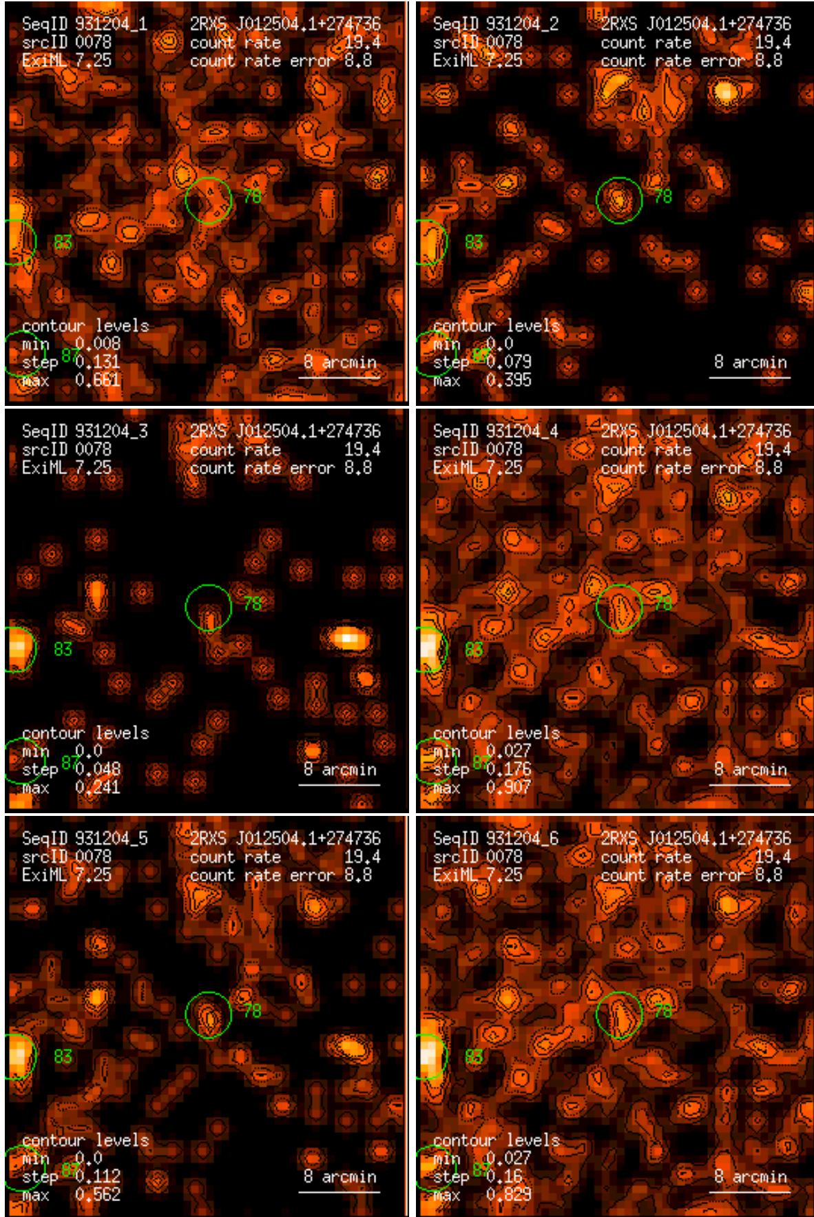
Figure 78: RASS 931204: detection 0078: band rate images, Gaussian filter: (1) PSPC channels 11 – 41, (2) 52 – 90, (3) 91 – 201, (4) 11 – 235, (5) 52 – 201, (6) 11 – 201. Broad band rates in counts/ks. Band rate contour levels in counts/ks/arcmin 2 .
