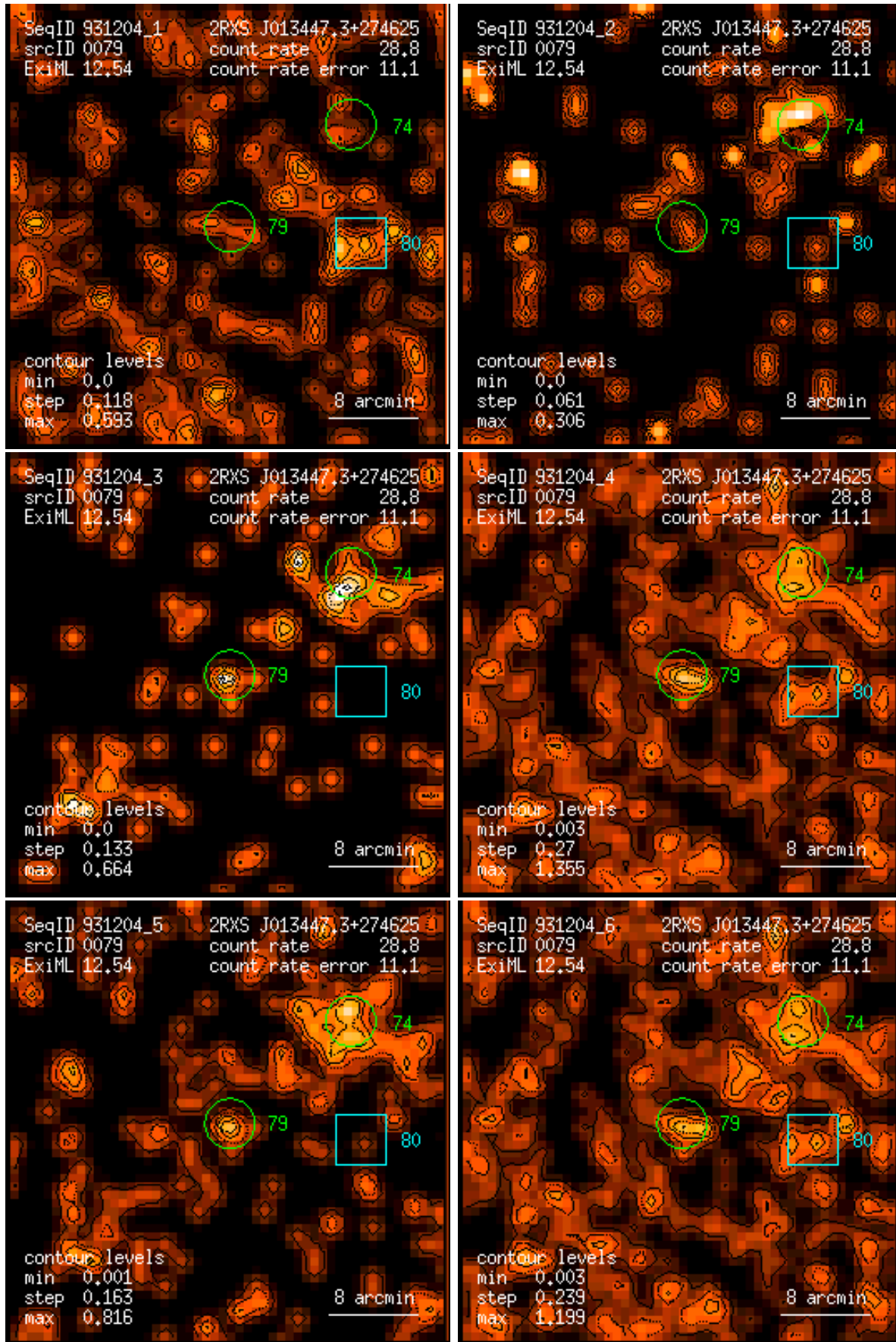
Figure 79: RASS 931204: detection 0079: band rate images, Gaussian filter: (1) PSPC channels 11 – 41, (2) 52 – 90, (3) 91 – 201, (4) 11 – 235, (5) 52 – 201, (6) 11 – 201. Broad band rates in counts/ks. Band rate contour levels in counts/ks/arcmin 2 .
