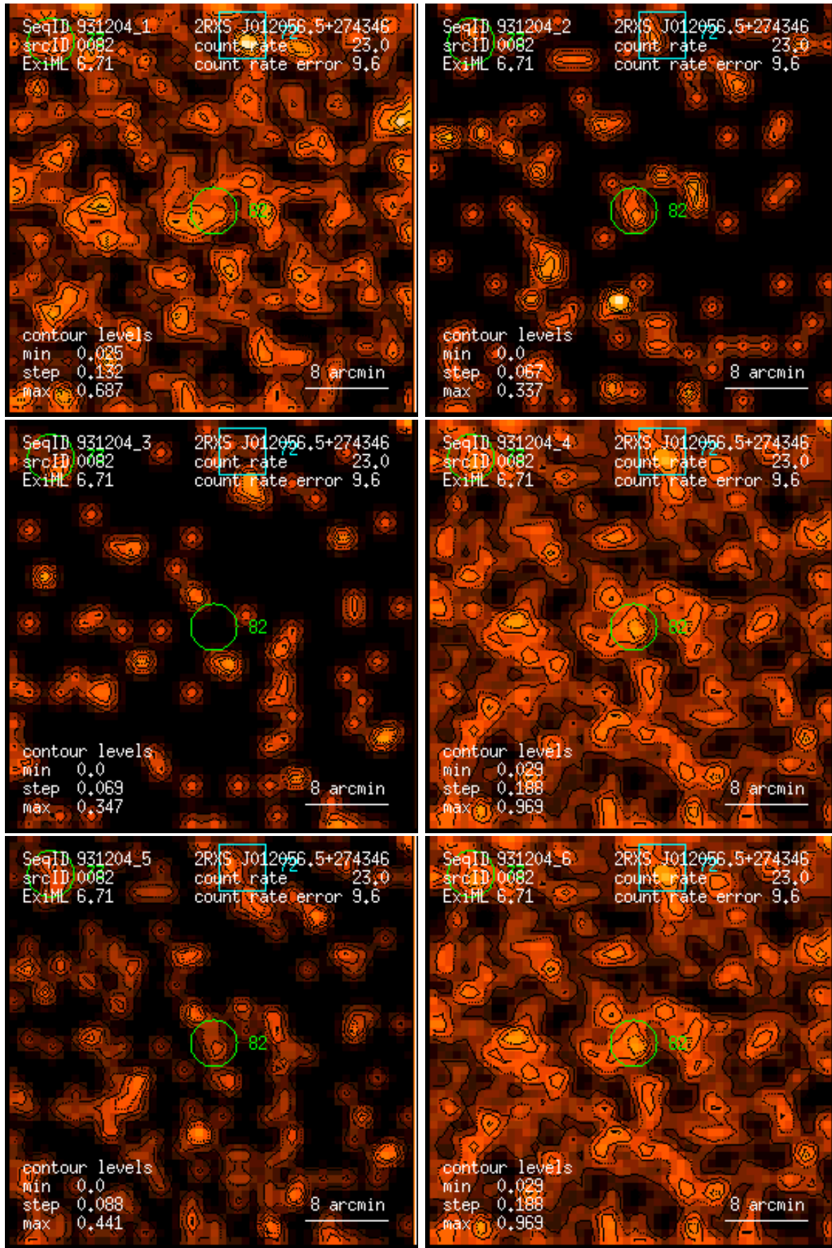
Figure 82: RASS 931204: detection 0082: band rate images, Gaussian filter: (1) PSPC channels 11 – 41, (2) 52 – 90, (3) 91 – 201, (4) 11 – 235, (5) 52 – 201, (6) 11 – 201. Broad band rates in counts/ks. Band rate contour levels in counts/ks/arcmin 2 .
