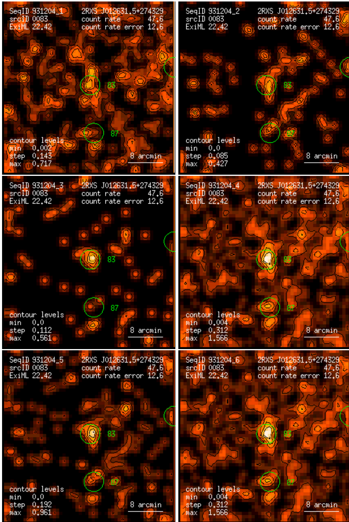
Figure 83: RASS 931204: detection 0083: band rate images, Gaussian filter: (1) PSPC channels 11 – 41, (2) 52 – 90, (3) 91 – 201, (4) 11 – 235, (5) 52 – 201, (6) 11 – 201. Broad band rates in counts/ks. Band rate contour levels in counts/ks/arcmin 2 .
